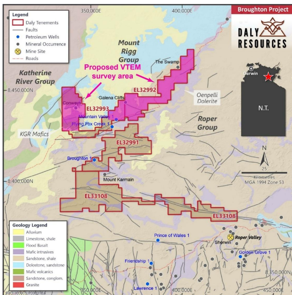
Figure 1. Broughton Project tenements showing regional geology, mineral occurrences and proposed VTEM survey areas.
