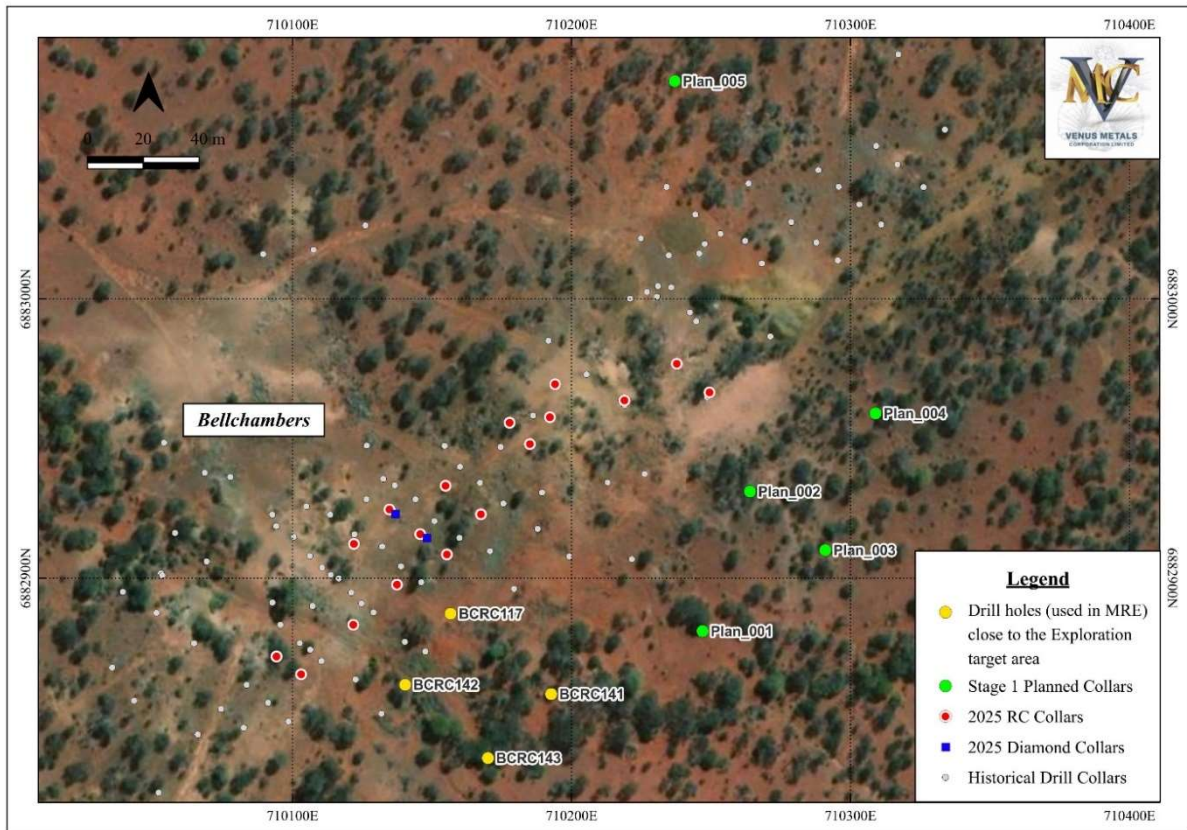
Figure 2. Location of the drilled holes at Bellchambers and planned drillholes (Plan 001-005) (phase 1) in Exploration Target Area
