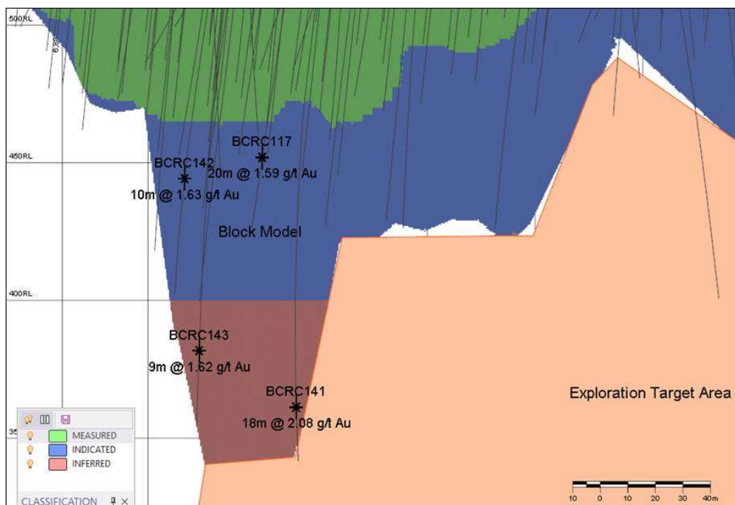
Figure 3. Long Section Detail of Exploration Target Area with Drill Hole Intersections relevant to estimating the Target parameters
