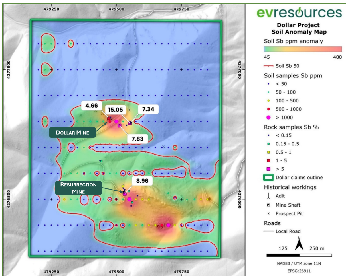
Figure 3: Dollar Project – Soil Anomaly Map- Antimony (ppm Sb) and Previously Reported Rock chip Results
