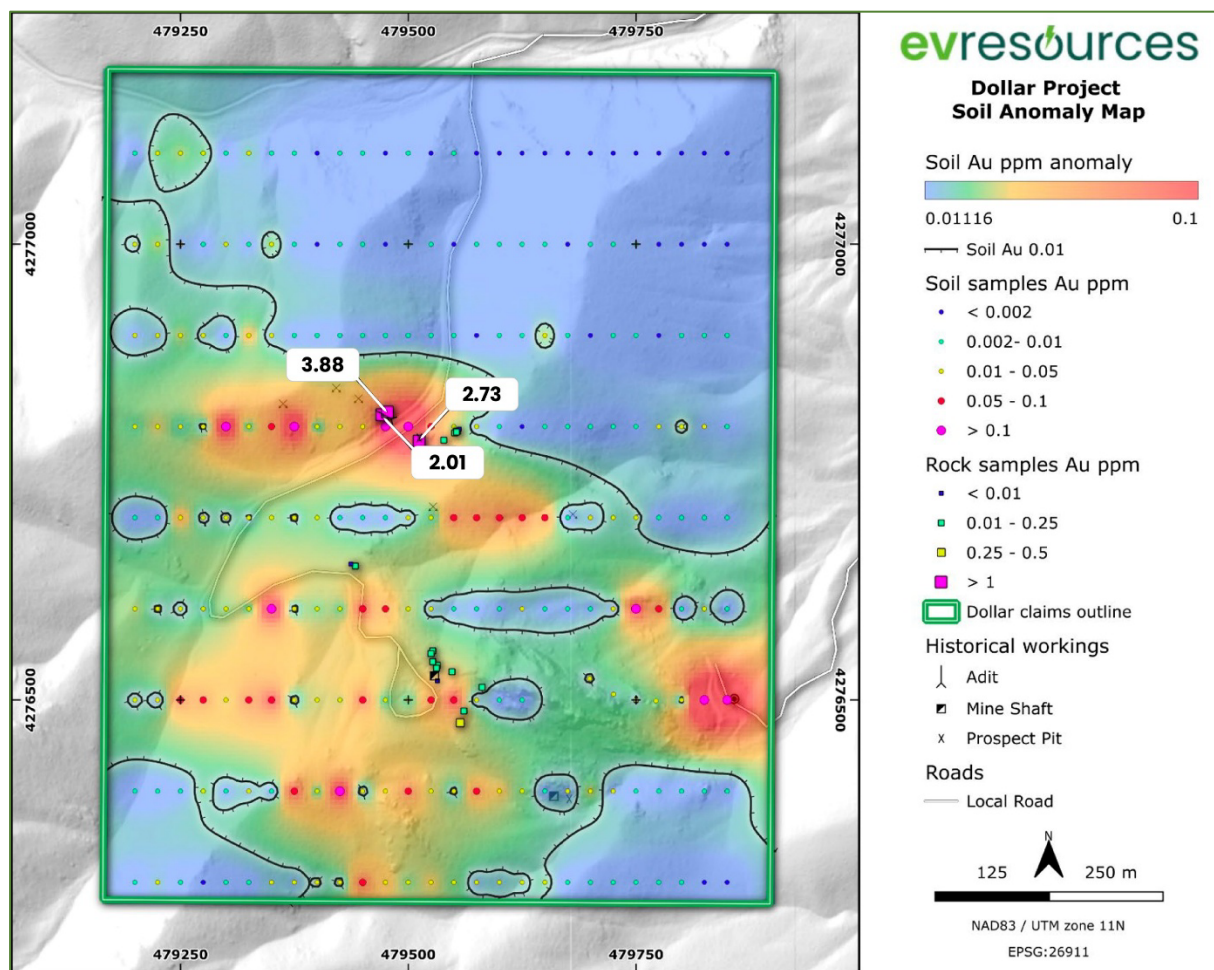
Figure 4: Dollar Project – Soil Anomaly Map- Gold (Au ppm) and Previously Reported Rock chip Results
