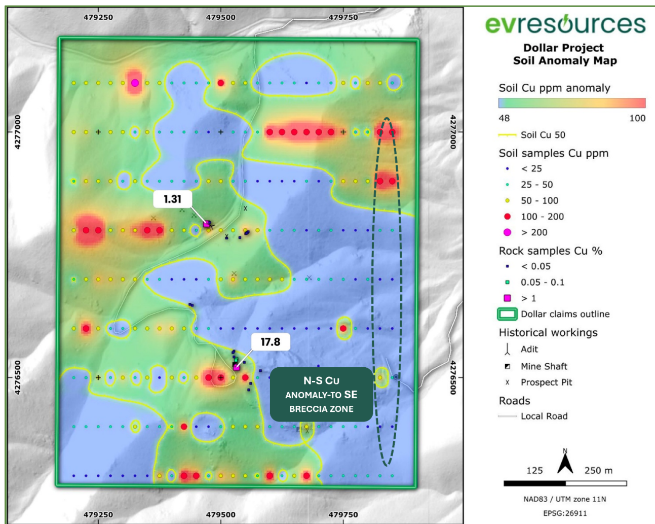
Figure 5: Dollar Project – Newly Identified Copper-Oxide Breccia Target and Previously Reported Rock chip Results
