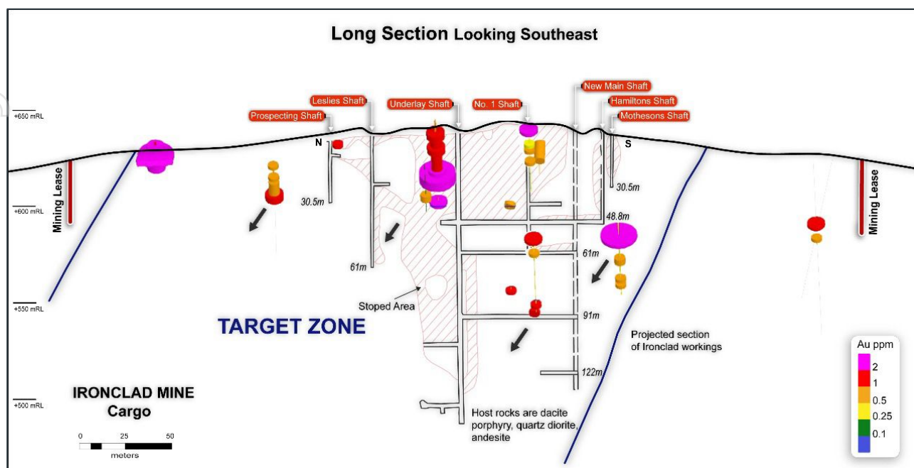
Figure 3: Ironclad Mining Lease, Schematic Long Section
