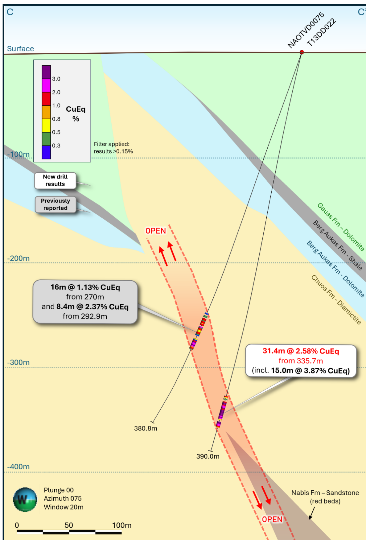
Figure 4: Cross section C-C' T-13 West Zone. 2
