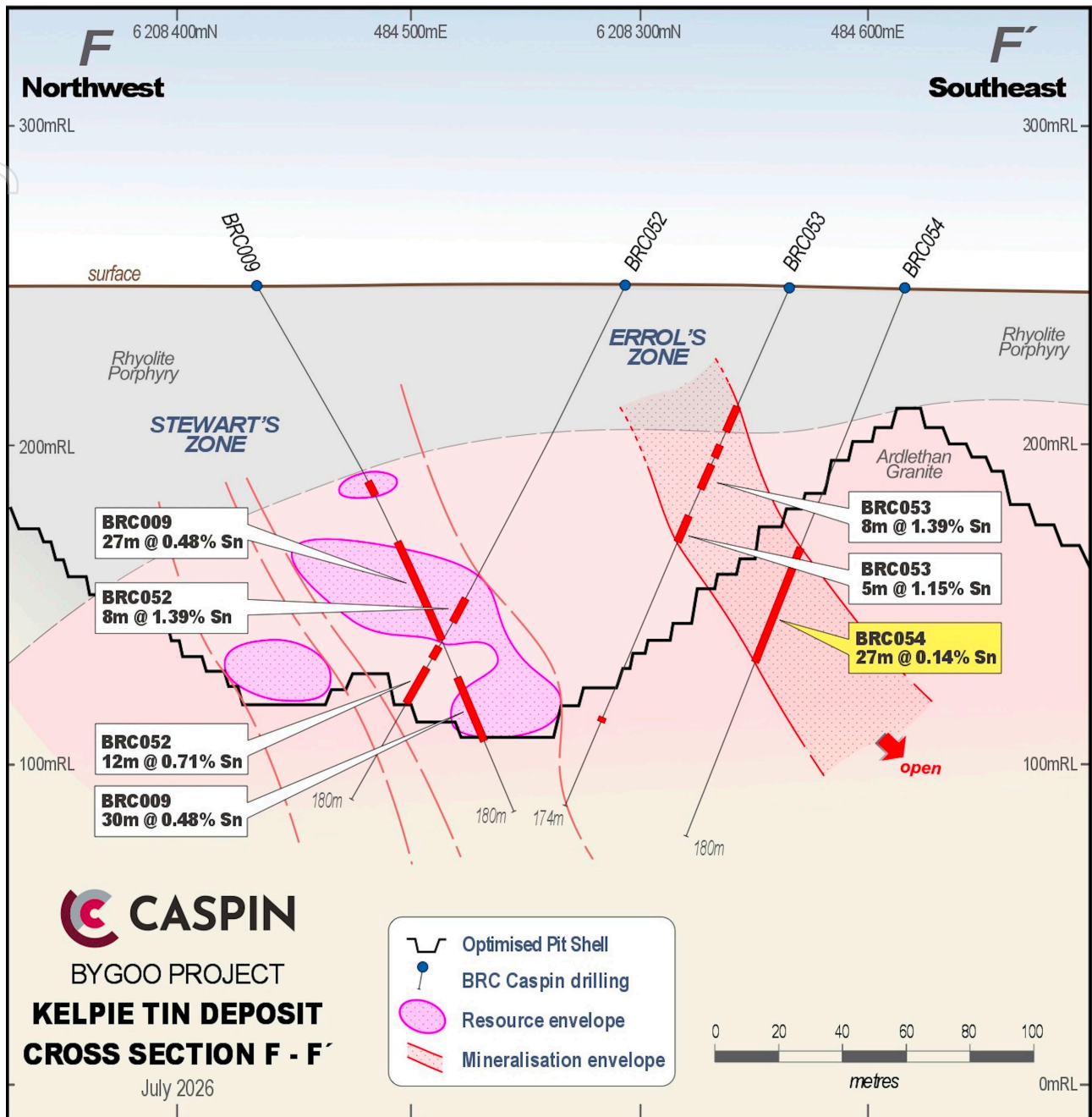
Figure 3. Cross section showing relationship between mineralisation on the Errol's and Stewart Fault Zones.
