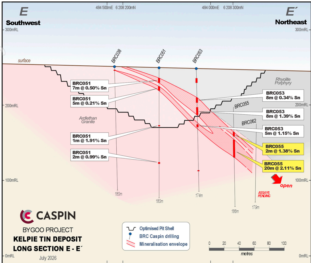
Figure 2. Long section of mineralisation on the Errol's Fault. Note that mineralisation is increasing in tenor and thickness along strike to the east. Results from BRC062 are pending.
