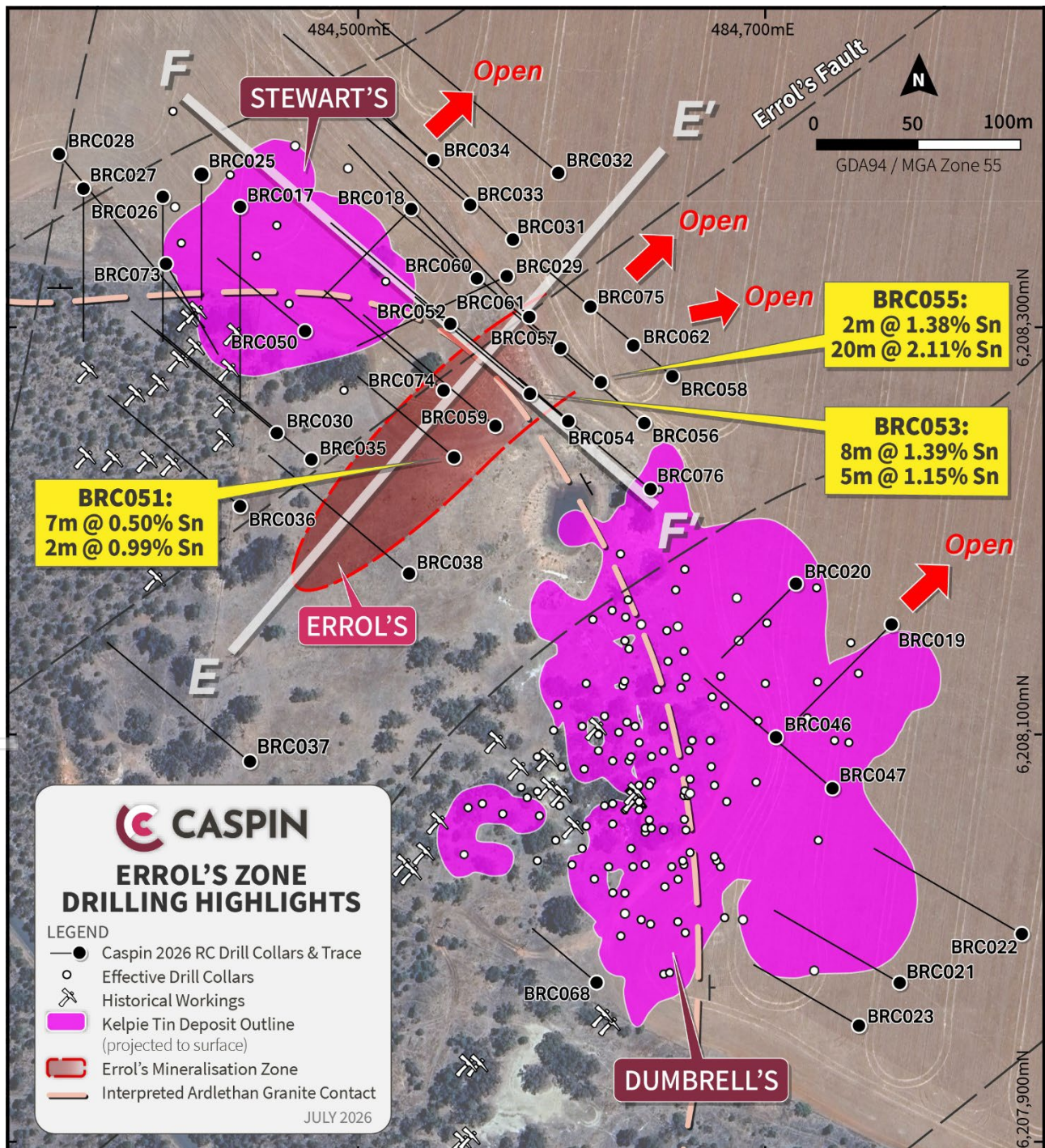
Figure 1. Kelpie drilling plan with significant Errol's Zone results and deposit outlines.
