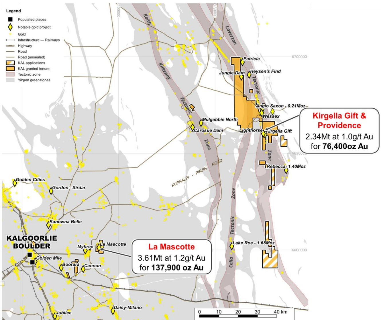
Figure 3 – Location map of the Kirkella Gift-Providence gold deposit and the Lighthorse prospect within KalGold's Pinjin Project, located around 140 km northeast of Kalgoorlie-Boulder. The project is situated approximately 25 km north of Ramelius Resources' (ASX: RMS) Rebecca Gold Project. Also shown is KalGold's outcropping La Mascotte gold deposit 35 km east of Kalgoorlie. Projection: MGA 94 Zone 51.
