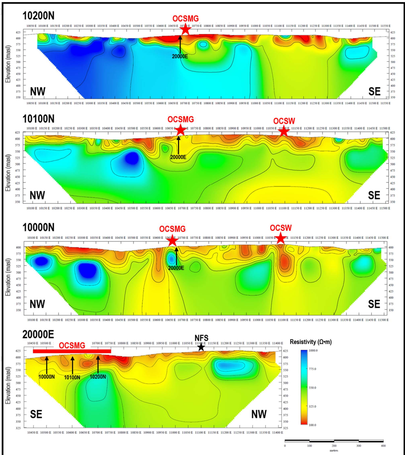
Figure 4: Modelled 2D resistivity sections for the four DDIP lines comprising Red Mountain's orientation IP survey at Oak Creek South. For line locations refer to Figure 1. All DDIP lines intersect the Oak Creek South Main Grid auger soil anomaly (OCSMG); Lines 10100N and 10000N intersect the Oak Creek South Workings auger soil anomaly and historical workings (OCSW); and Line 20000E intersects the Namoi Fault Splay (NFS), where shown. The points where Line 20000E intersects the three NW-SE trending lines and the intersections of those lines on Line 20000E are also indicated by the black vertical arrows.
