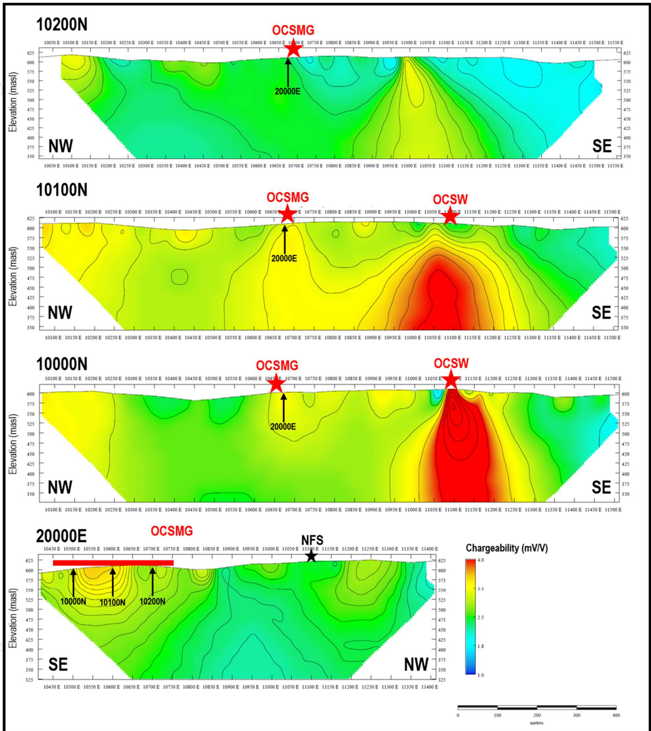
Figure 2: Modelled 2D chargeability sections for the four DDIP lines comprising Red Mountain's orientation IP survey at Oak Creek South. For line locations refer to Figure 1. All DDIP lines intersect the Oak Creek South Main Grid auger soil anomaly (OCSMG); Lines 10100N and 10000N intersect the Oak Creek South Workings auger soil anomaly and historical workings (OCSW); and Line 20000E intersects the Namoi Fault Splay (NFS), where shown. The points where Line 20000E intersects the three NW-SE trending lines and the intersections of those lines on Line 20000E are also indicated by the black vertical arrows.
