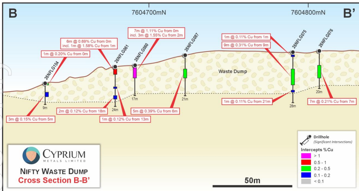
Figure 5: Cross section B-B' through the Nifty waste dump
