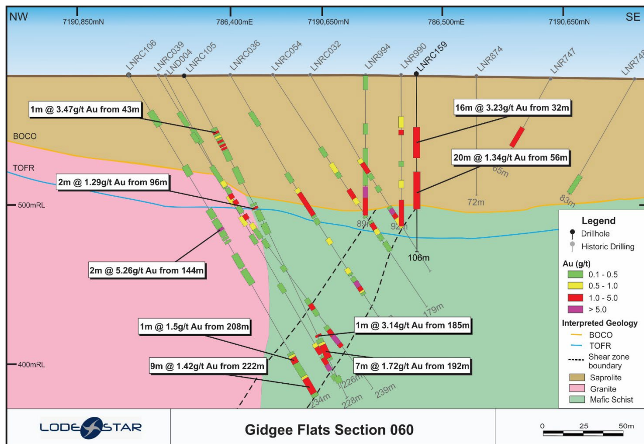
Figure 3: Gidgee Flat - Cross Section of Hole LNRC159
