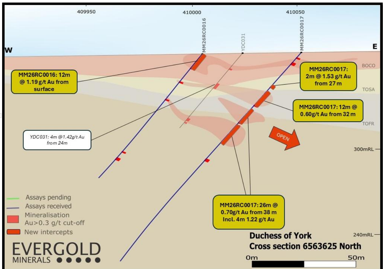
Figure 2: Representative cross-section through Duchess of York 1 . MM26RC0016-018
