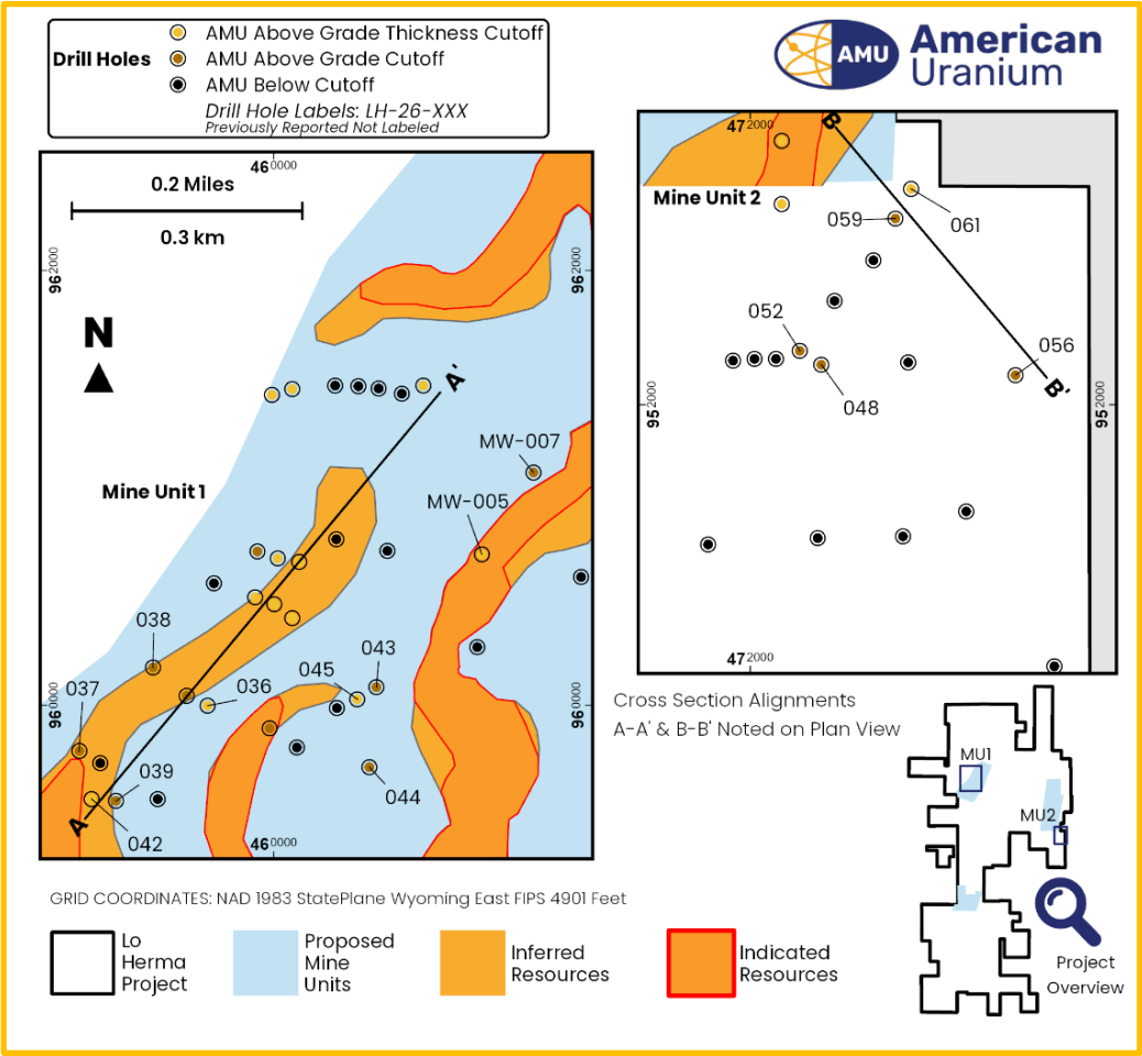
FIGURE 2: DRILL HOLE COLLAR MAPS, MINE UNITS 1 AND 2
