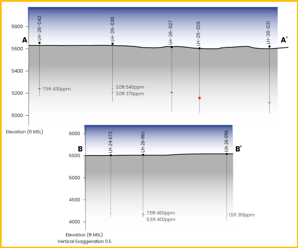
FIGURE 3A: CROSS SECTION OF MINERALISED DRILL HOLE INTERCEPTS
