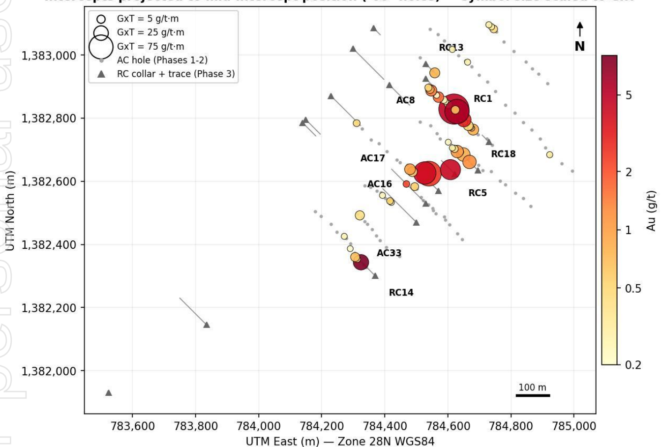
Figure 2 – Plan view of combined Phase 1-2 Aircore and Phase 3 RC gold intercepts (0.2 g/t Au cutoff); symbol size scaled to grade-thickness (GxT, g/t-m), colour scaled to gold grade.
