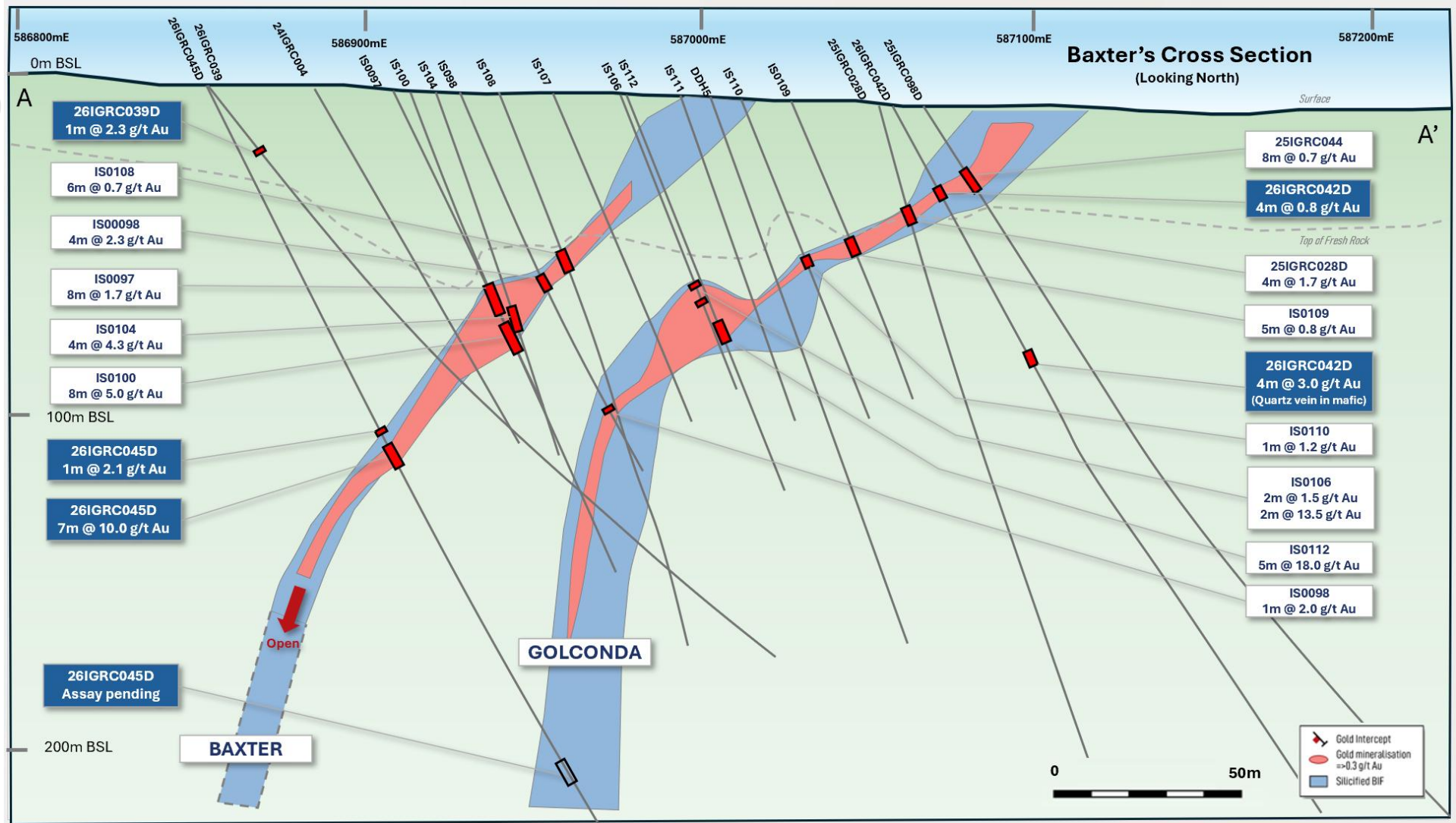
Figure 3: Schematic cross section of Baxter showing new drill intersections (blue boxes).
