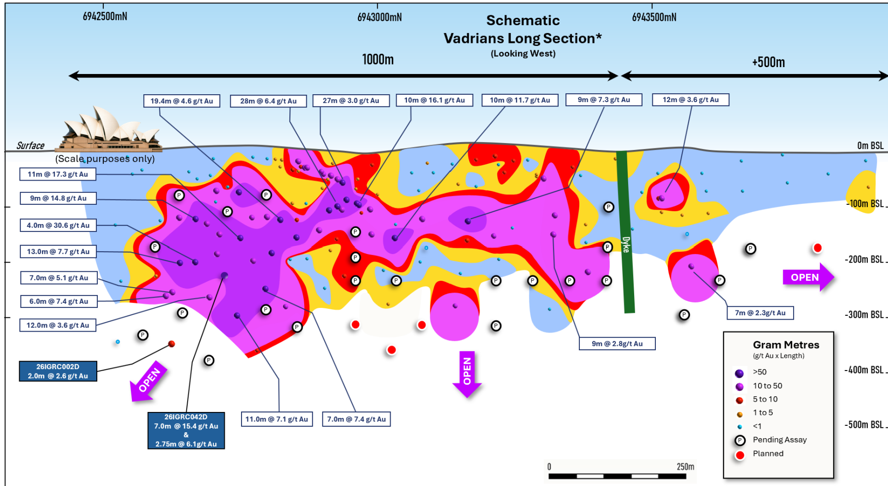
Figure 1: Schematic long section of the Vadrians gold deposit showing new drill intersections (blue boxes) with gold gram-metre contour interpretation.
