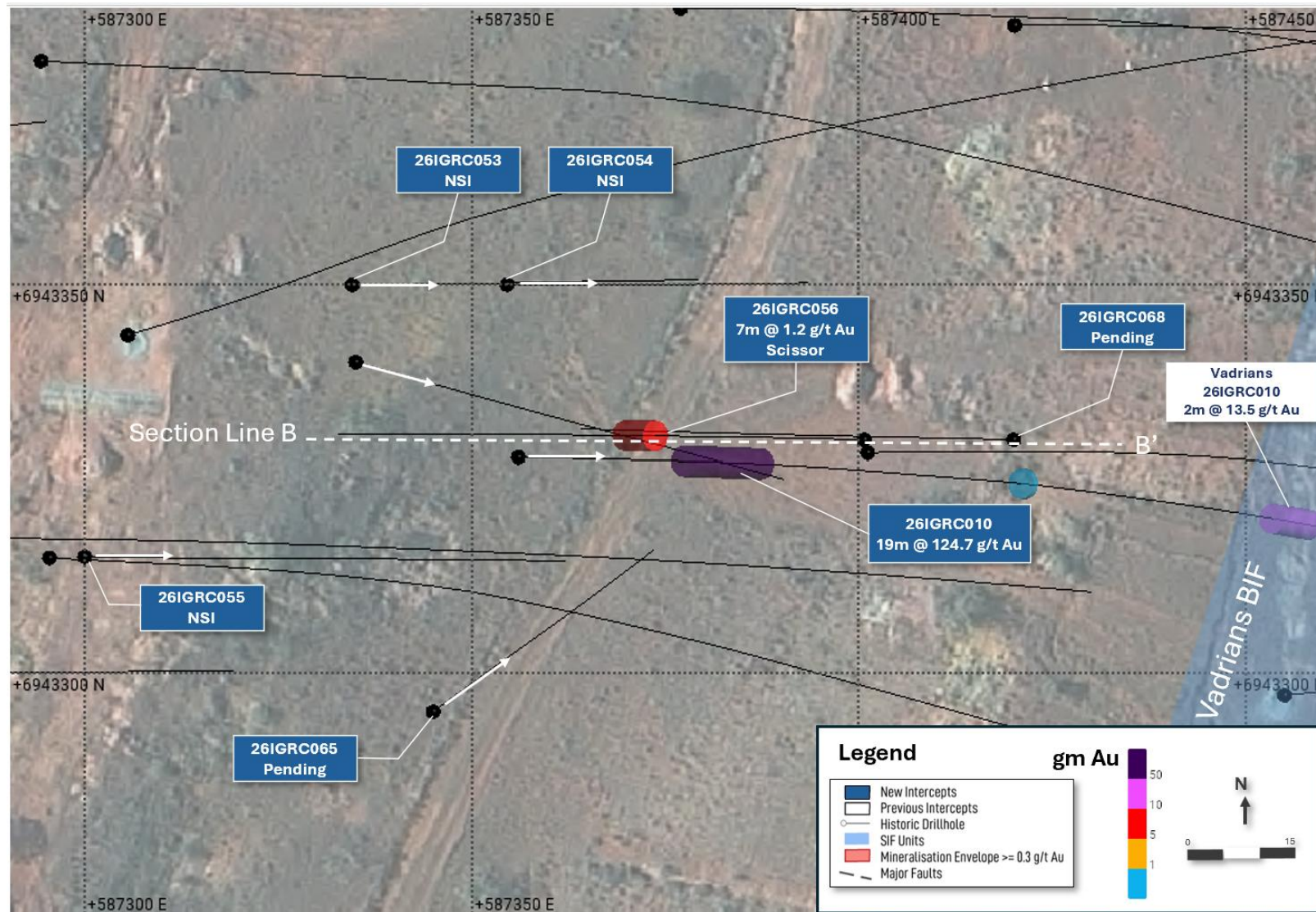
Figure 5: Schematic plan of the Bonanza grade in drill hole 26IGRC010 and close spaced drilling showing new drill intersections (blue boxes).
