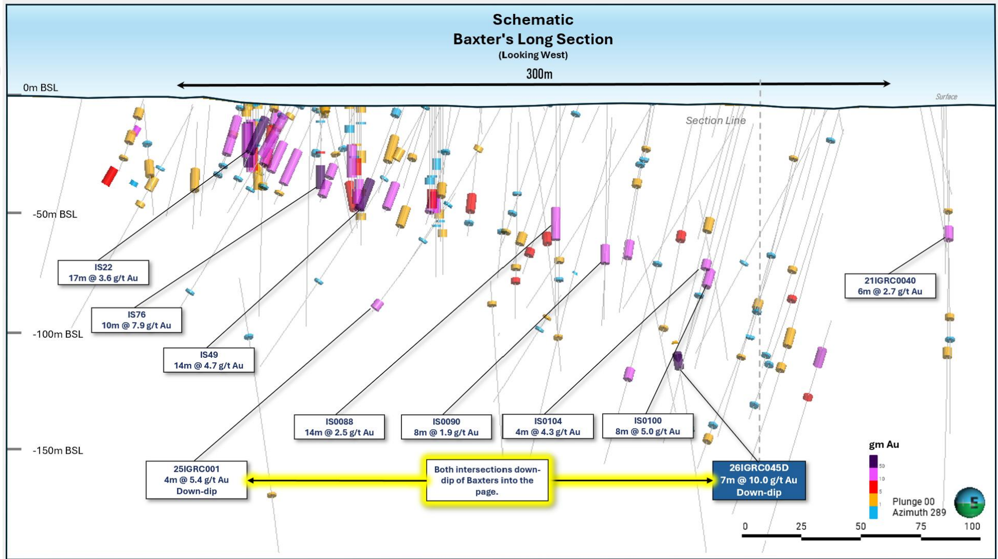
Figure 2: Schematic long section of the Baxter gold deposit showing new drill intersections (blue boxes) with gold gram-metre intersections.
