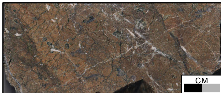
Figure 7: SPD052 – 301.6 m, 58.47 g/t Au. Basalt with early quartz-pyrite alteration overprinted by intense potassic alteration with strong disseminated and pyrite stringers with late carbonate breccia adjacent to fault zone.
