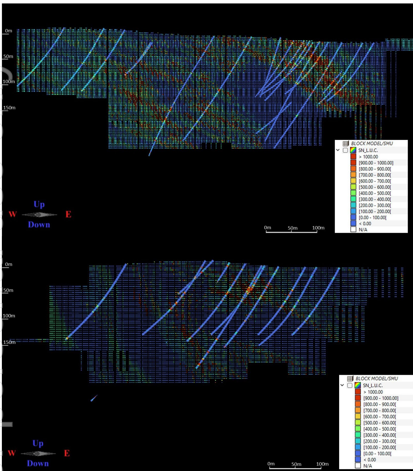
Figure 6: Cross sections of 1m composites and the estimated Sn grades. The sections are 40 m thick.
