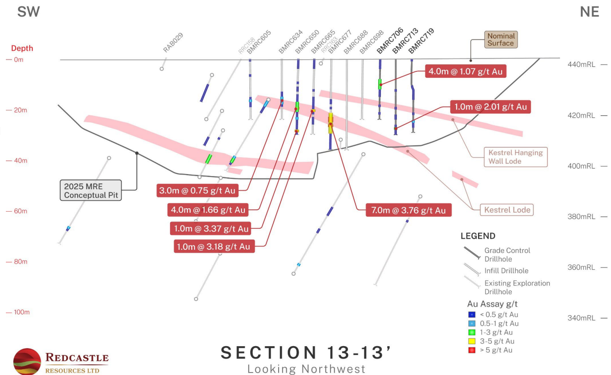
Figure 13. Queen Alexandra Section 13-13'
