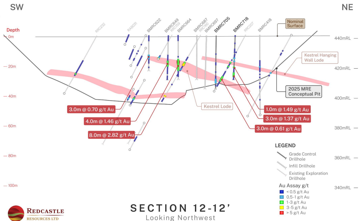
Figure 12. Queen Alexandra Section 12-12'
