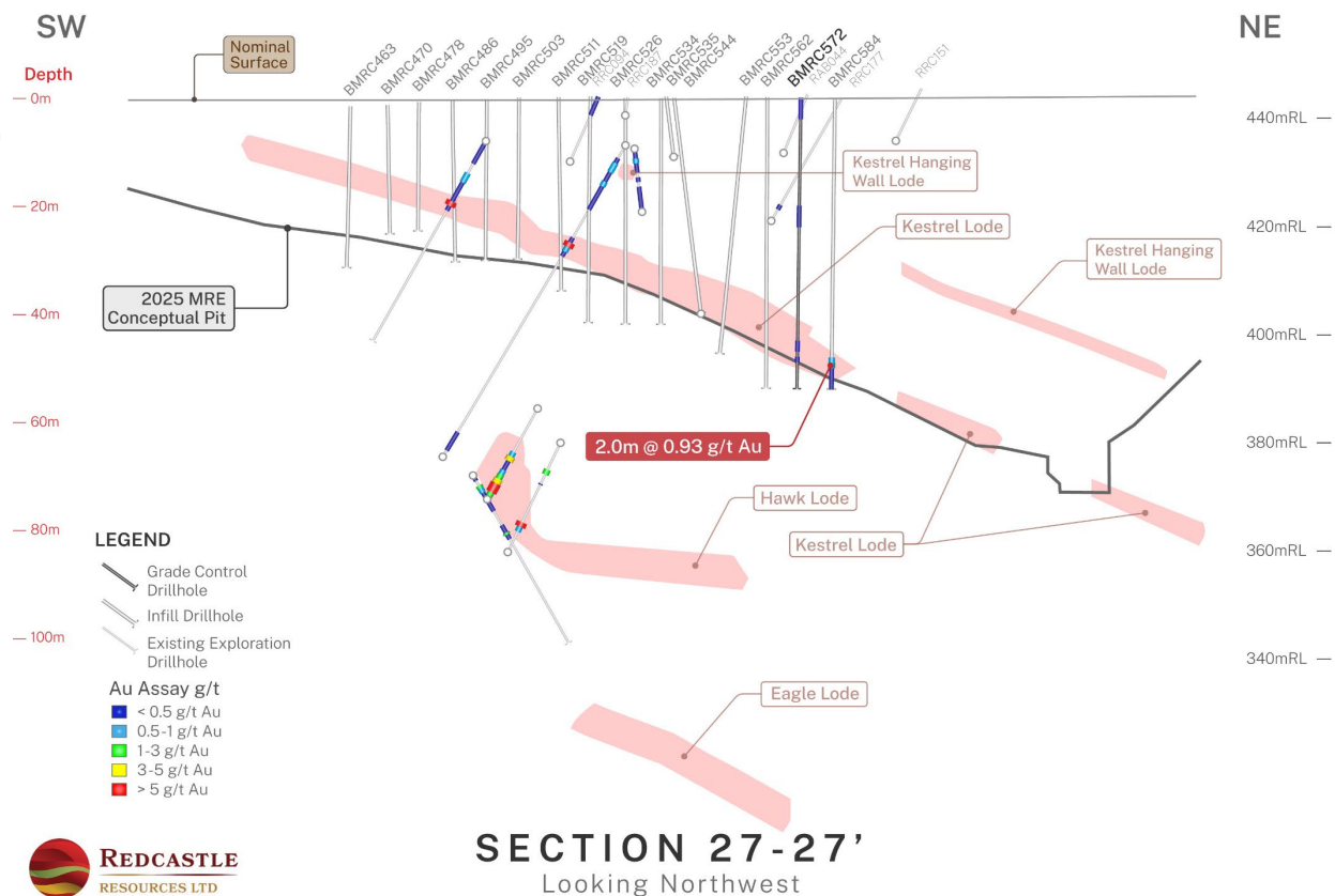
Figure 22. Queen Alexandra Section 27-27'
