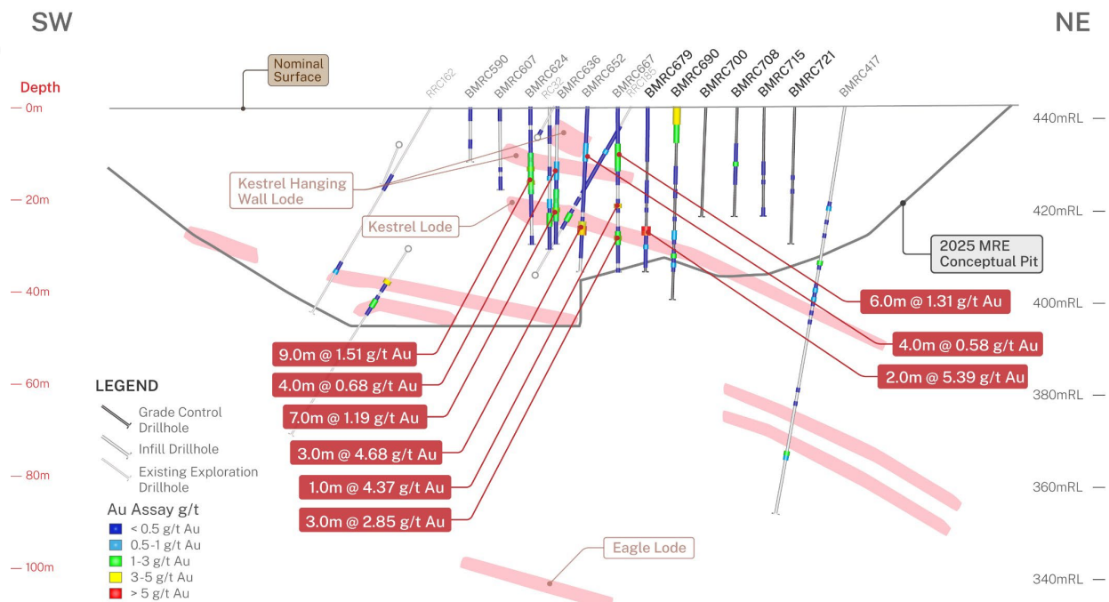
SECTION 15-15' Looking Northwest Figure 4. Queen Alexandra Section 15-15'
