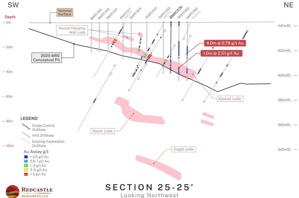
Figure 20. Queen Alexandra Section 25-25'
