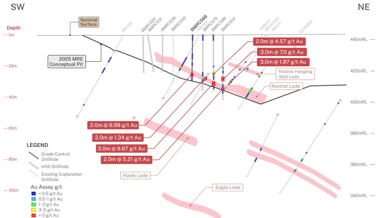
Figure 18. Queen Alexandra Section 21-21'
