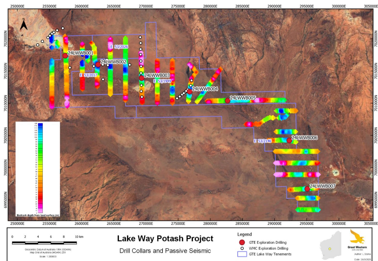
Figure 10: Position of reported drill-holes at the Lake Way Potash Project ((GTE ASX Announcement 9 March 2025), overlaid on previously reported passive seismic sections ((GTE ASX Announcement 22 May 2023) and satellite imagery. Note drill-holes 24LWWB004 to 24LWWB007 are interpreted to be offset to the channel's thalweg, with re-drilling targeting the central position interpreted to potentially double channel's length.
