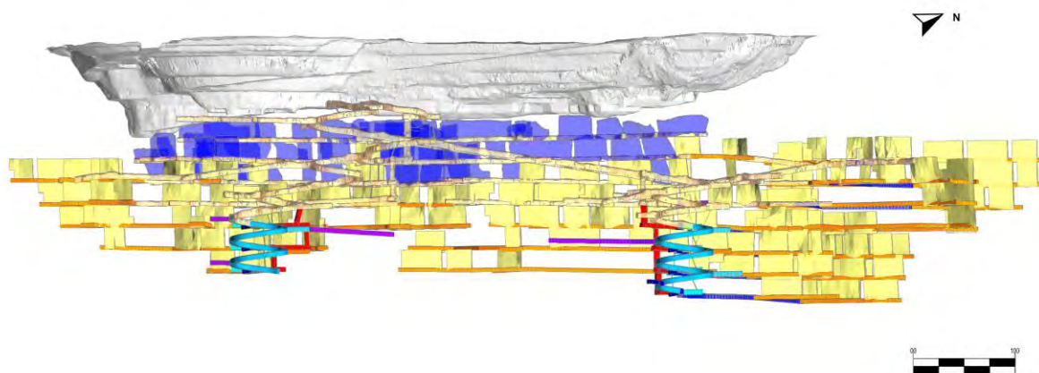
Figure 8 - Sand King Underground Ore Reserve mine design with Sand King pit (looking northwest)
