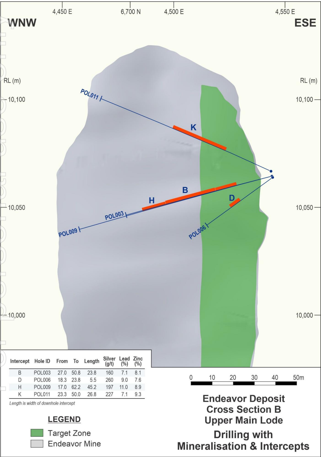
Figure 4. Cross Section B – Upper Main Node drilling with mineralised intercepts.
