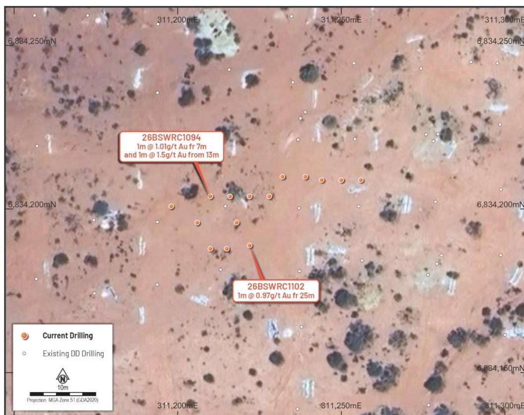
Figure 3 – Plan View of Grade Control Inset 2 at Mt Stirling Well Gold Deposit with significant Intercepts
