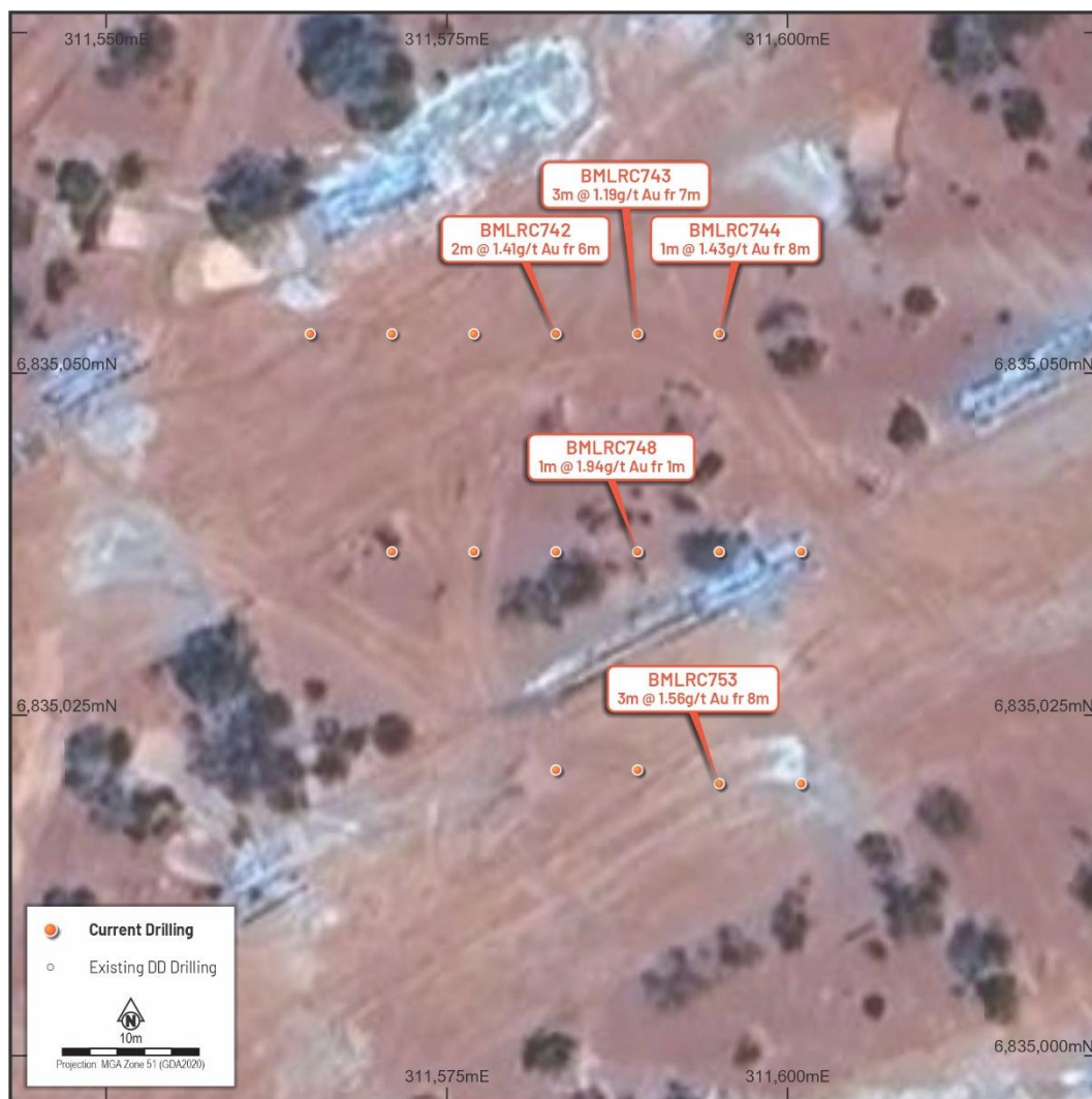
Figure 5 – Plan View of Grade Control at Mt Stirling Gold Deposit with significant Intercepts
