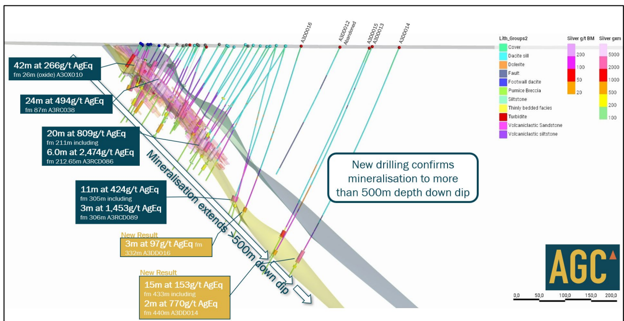
Figure 1: Achilles northern zone cross section looking north through 6,329,070N showing high grade mineralisation from surface to 540m down dip depth.
