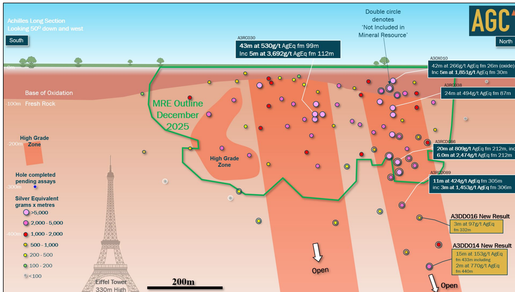
Figure 3: Achilles schematic long section showing drill hole pierce points coloured by silver equivalent x metres and new results in yellow boxes. Double circle denotes holes that were not included in the MRE. See silver equivalent disclosures section.
