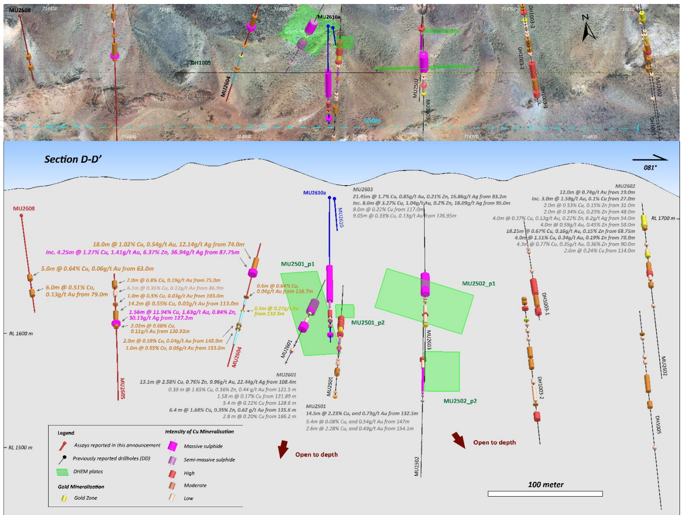
Figure 4. Longitudinal section along copper mineralisation zone.
