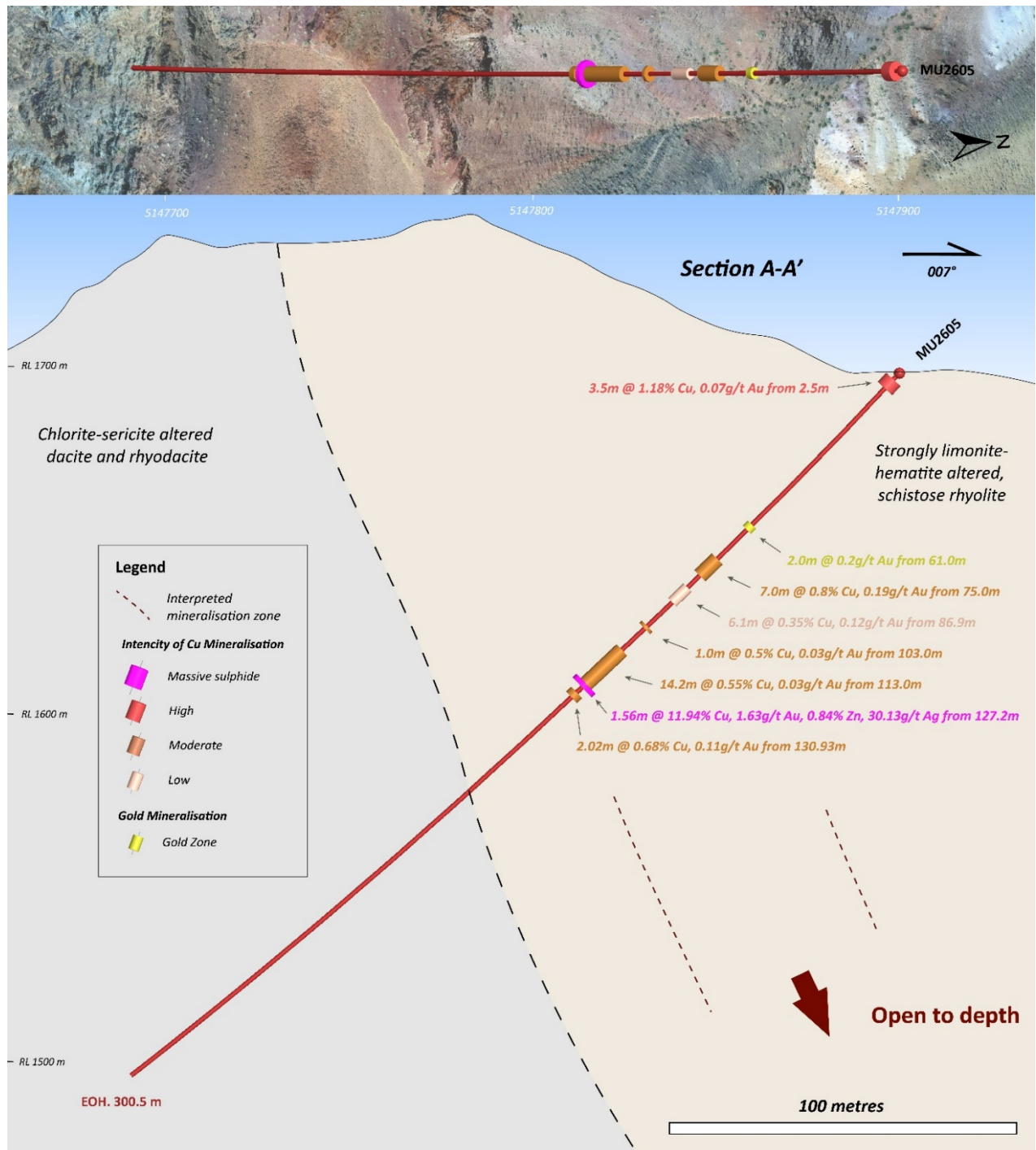
Figure 2. Cross section along drillhole MU2605
