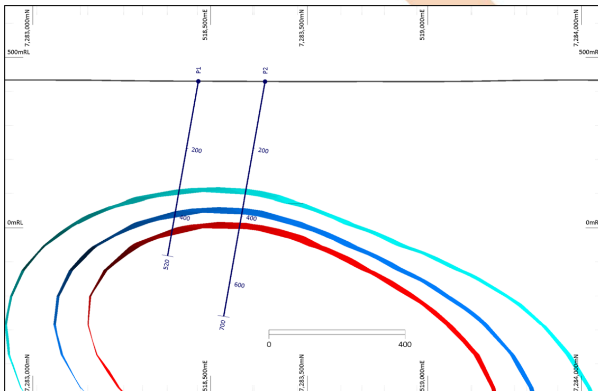
Figure 5: Magnetic inversion modelling of the Madman. The image (cross section looking NW) illustrates the proposed exploration program, consisting of 2 deep drill holes (see Figure 4 for cross section location). The inversion models were produced using the Magnetic Vector Inversion technique and represent contours of 5 (l blue), 10 (dark blue) and 15 (red) \text{SI} \times 10^{-3} . Hole MD002DD follows the trace of hole P1, and has not intersected sufficiently magnetic material to explain the anomaly (see Table 2), which Buxton now interprets to lie to the North in the area of planned hole P2.
