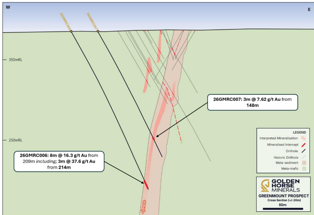
Figure 3: Cross section looking North (A – A') denoting high-grade intersection within hole 26GMRC006: 8m @ 16.3 g/t Au from 209m and hole 26GMRC007: 3m @ 7.62 g/t Au from 148m.
