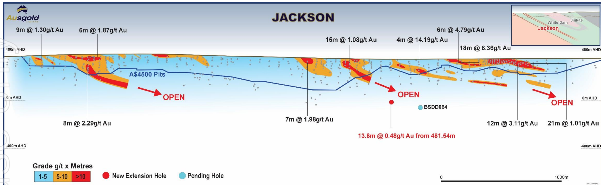
Figure 7 – Jackson trend long-section looking WSW displaying gram-metre contours (0.3g/t Au cut-off), pierce points of existing drilling, DHEM plates, pit optimisation (A$4,500 Resource constraint) and zones of ongoing drilling
