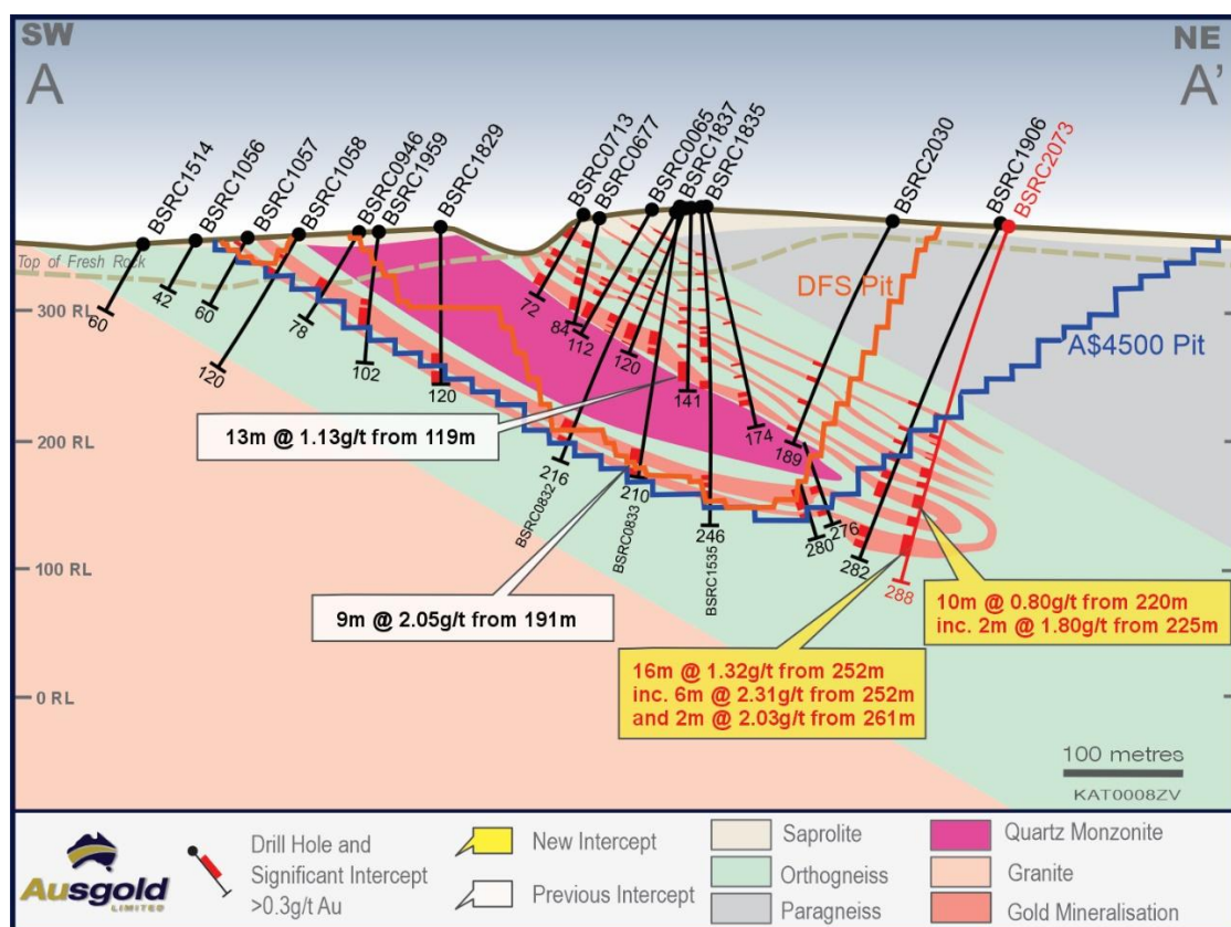
Figure 3 – Cross-section A-A' across the Jinkas-White Dam Lodes with current drilling program results (note that the A$4500/oz Resource pit shells above and below were determined based on available drill data at the time – all drill holes displayed provide new data which will be factored into the next Mineral Resource update)
