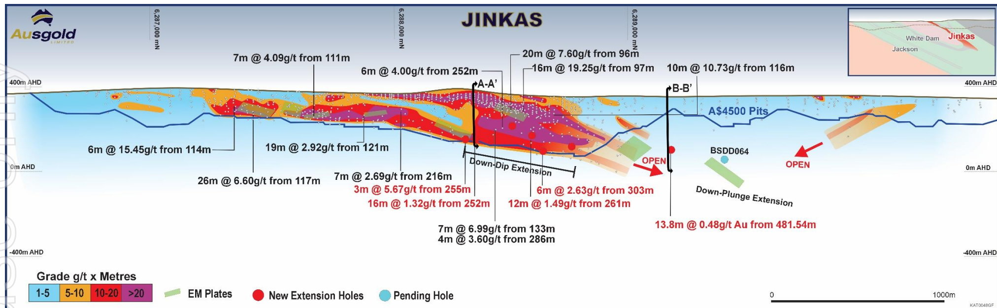
Figure 6 – Jinkas trend long-section looking WSW displaying gram-metre contours (0.3g/t Au cut-off), pierce points of existing drilling, new extension drilling, pending drilling, DHEM plates and pit optimisation (A$4,500 Resource constraint)
