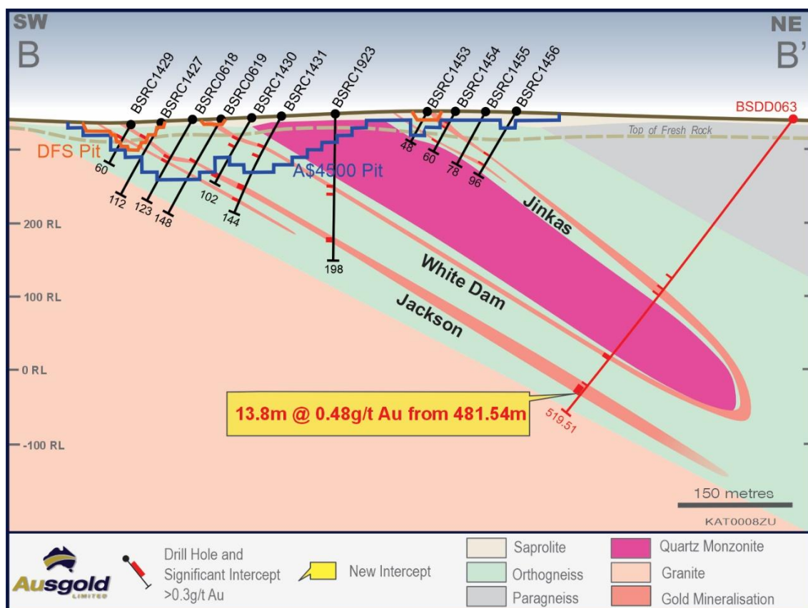
Figure 4 – Cross-section B-B' across the Jinkas-White Dam and Jackson Lodes with Resource drilling and Pits
