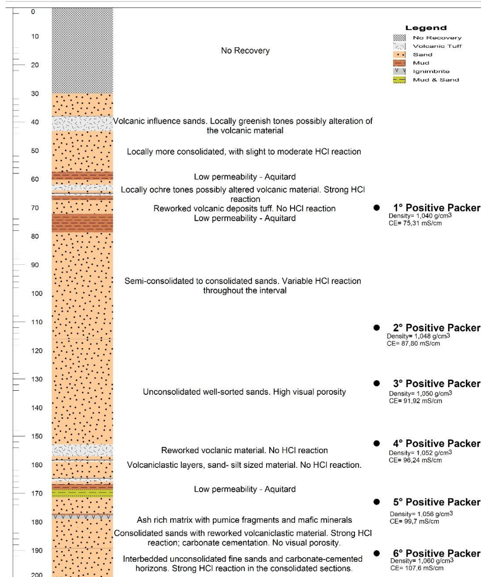
Figure 1. JAM 26-08 Cilon lithology column showing brine assay with porous sands and packer field measurements.
