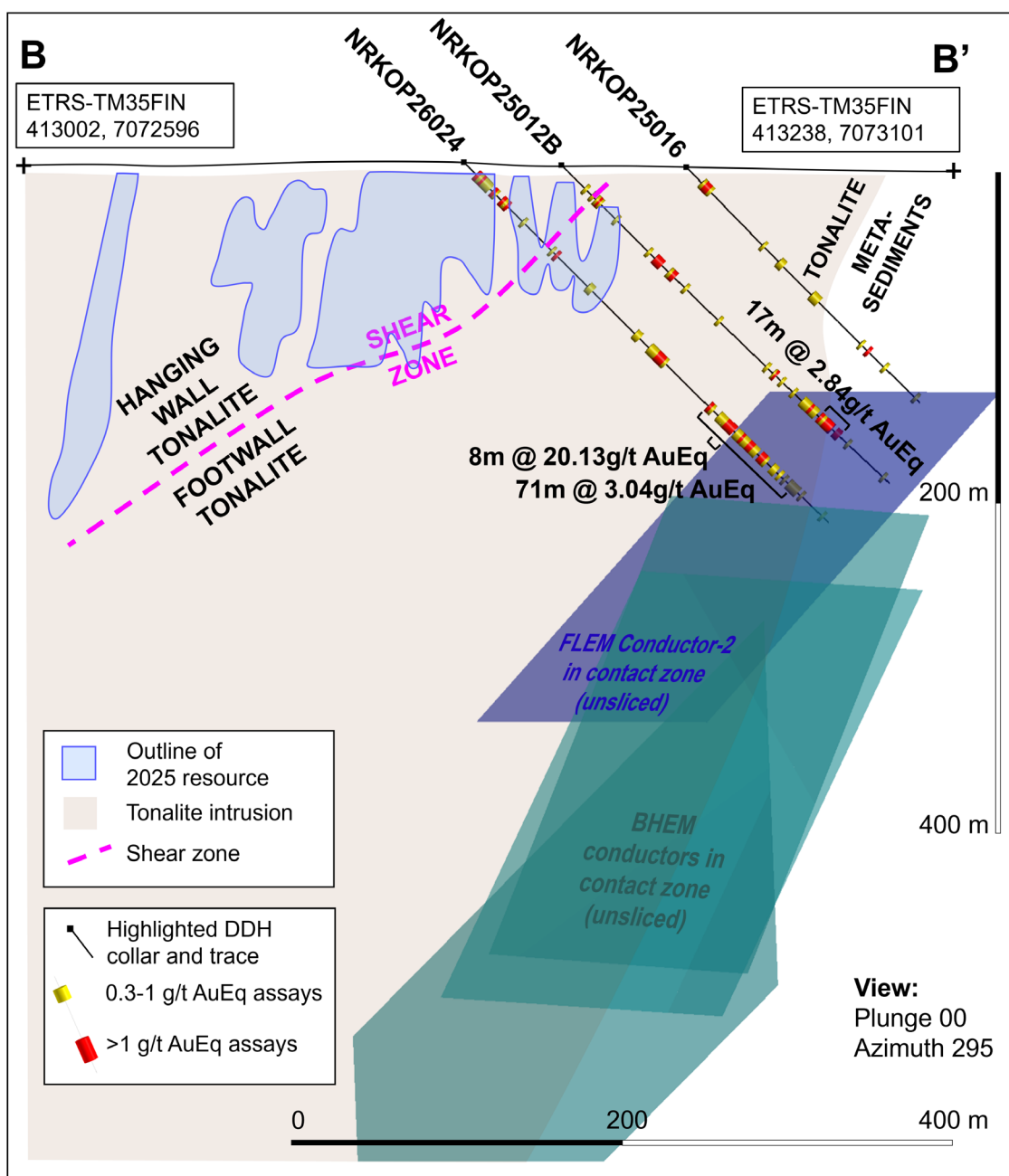
Figure 4: Kopsa cross section B showing holes NRKOP25016, NRKOP25012B and NRKOP26024. The most recent MRE outline, the interpreted extent of the tonalite intrusion and the previously modelled EM plates are also shown in this 30m thick section view. The EM plates are shown in their entirety to 600m vertical depth and not sliced to 30m thickness. See earlier ASX Announcement 7 for the full drill hole details. Coordinates presented in ETRS-TM35FIN system (EPSG:3067).
