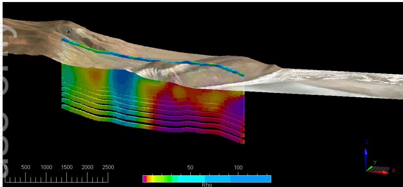
Figure 4 – CSAMT Cross Section (N3000) Showing DDH-3 Targeting the Core of the High-Conductivity Brine System
