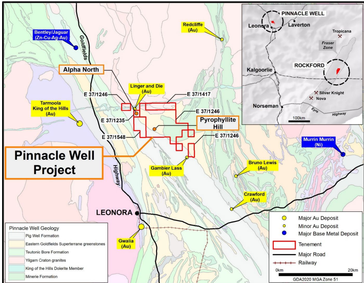
Figure 2: Pinnacle Well Project location with major mines/deposits on regional geology (GSWA 1:500K)
