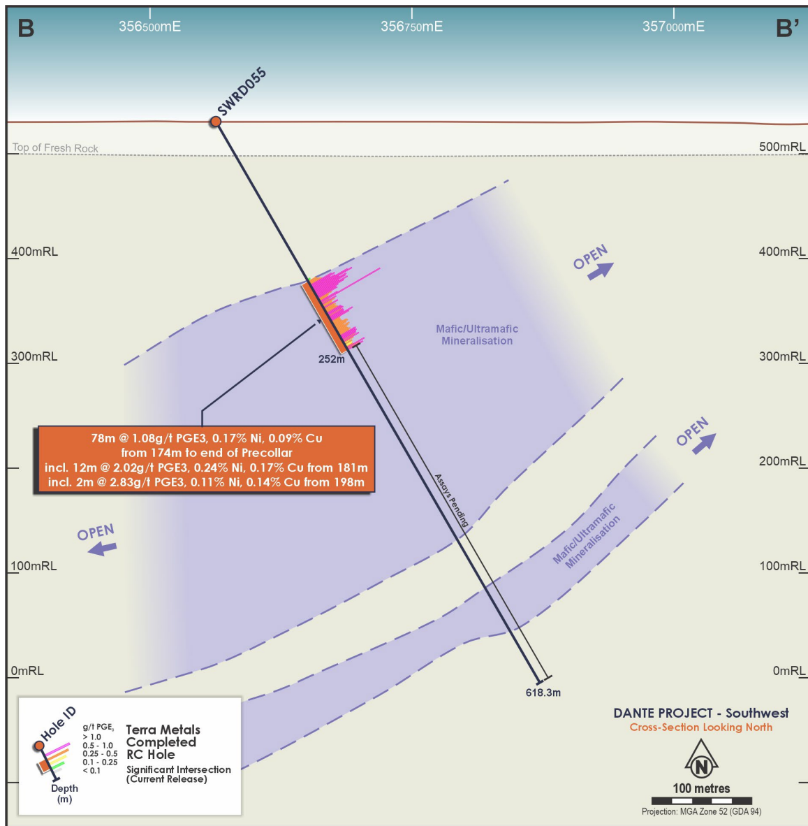
Figure 2. Cross-section B–B' through the Southwest Main Sulfide Zone showing the currently reported RC Pre-collar of SWRD055 with interpreted mineralised envelopes. The envelopes are conceptual and based on current drilling, geological logging and structural data.
