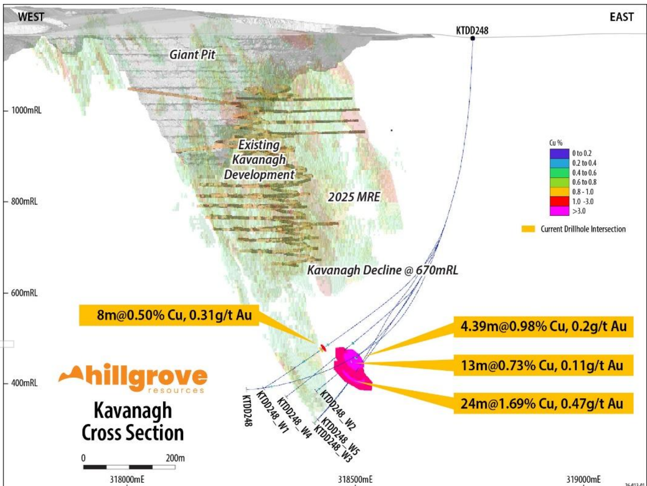
Figure 4: View towards the North showing significant intersections in relation to the 2025 MRE and existing Underground Development
