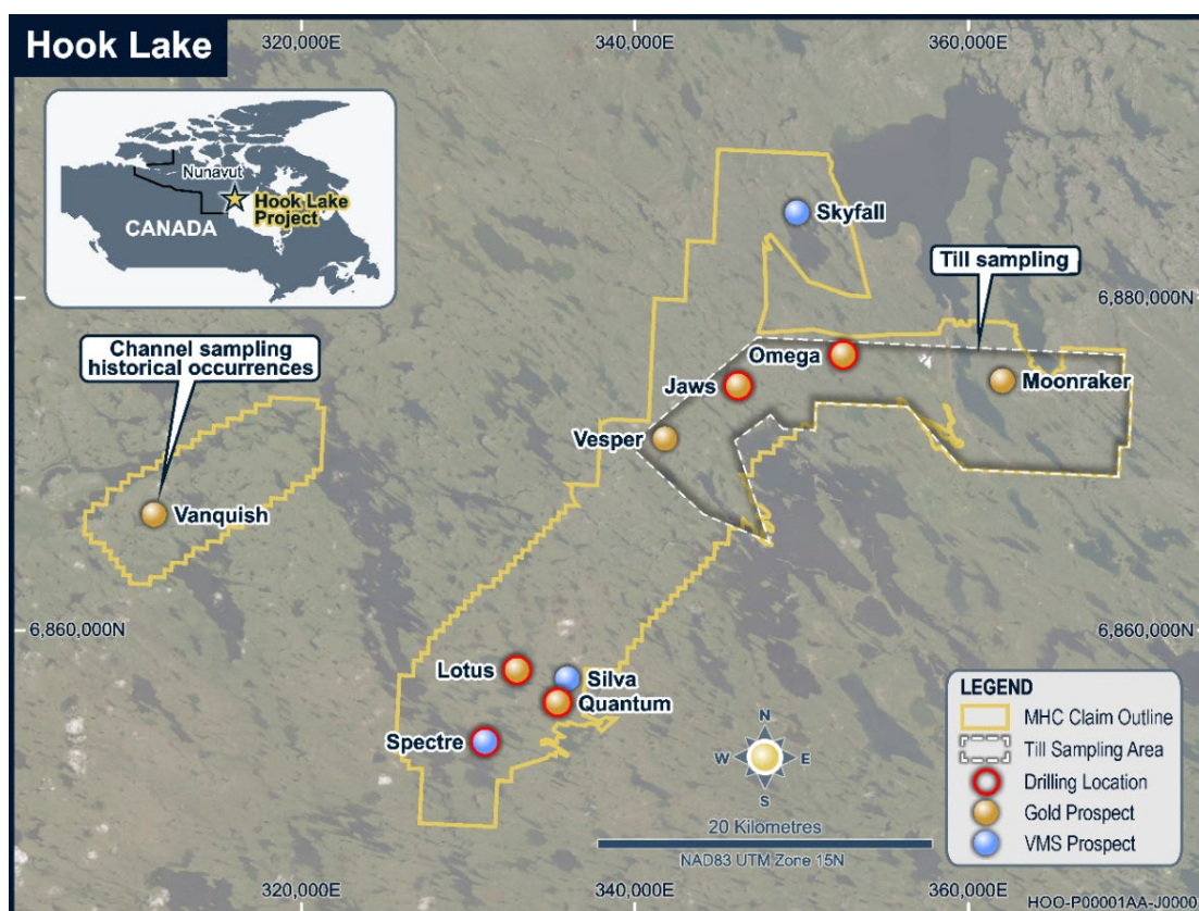
Figure 1: Hook Lake 2026 exploration program area with key gold and volcanogenic massive sulphide (VMS) prospects.
