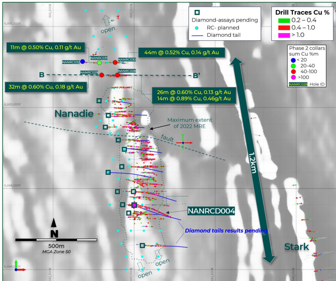
Figure 4. Nanadie Deposit aeromagnetic imagery and downhole copper values in previous drilling 1,2,4,5 projected to surface, showing the location of RC drillholes reported over the Quarter, drillholes extended with diamond tails (labelled), and current completed and planned Phase 2 RC drill collars (blue dots).
