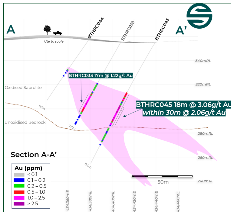
Figure 10: Bluetooth Gold Prospect cross-section A-A' (see Figure 5) showing Solstice's RC gold intercepts (white text) 9 .
