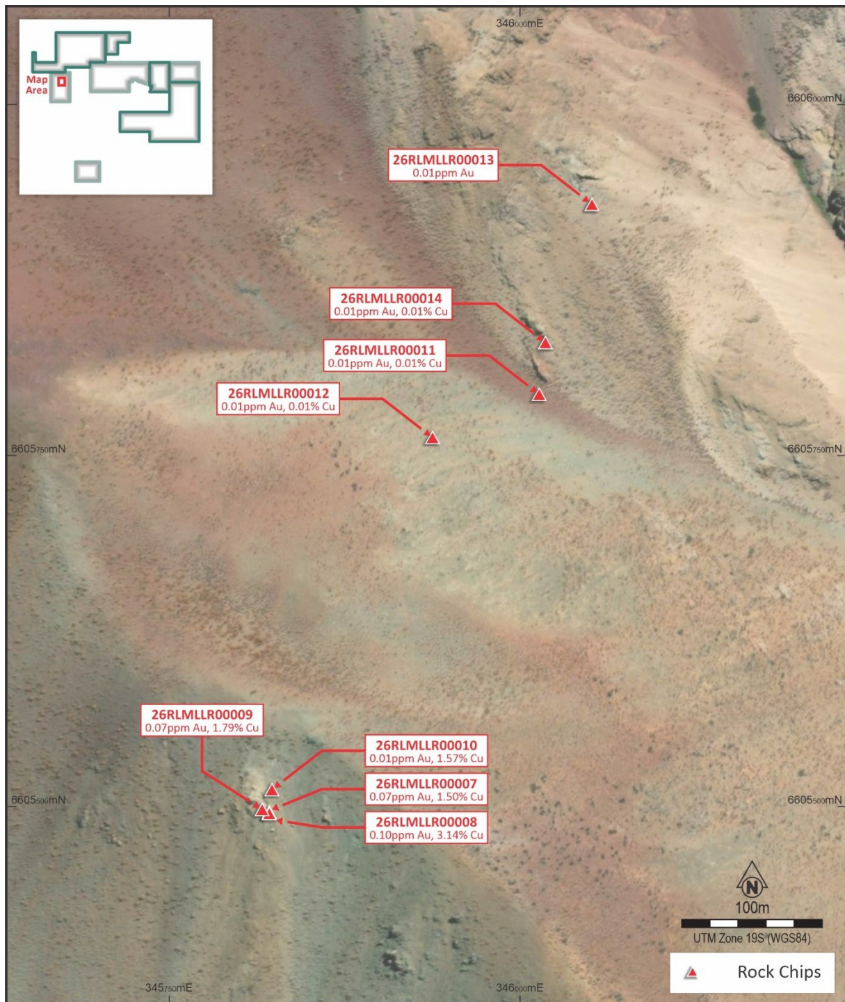
Figure 4. Inset map, showing higher resolution of the rock chip samples taken ~6km west of the Los Molles Prospect artisanal mining workings, along the same prospective carbonate horizon.
