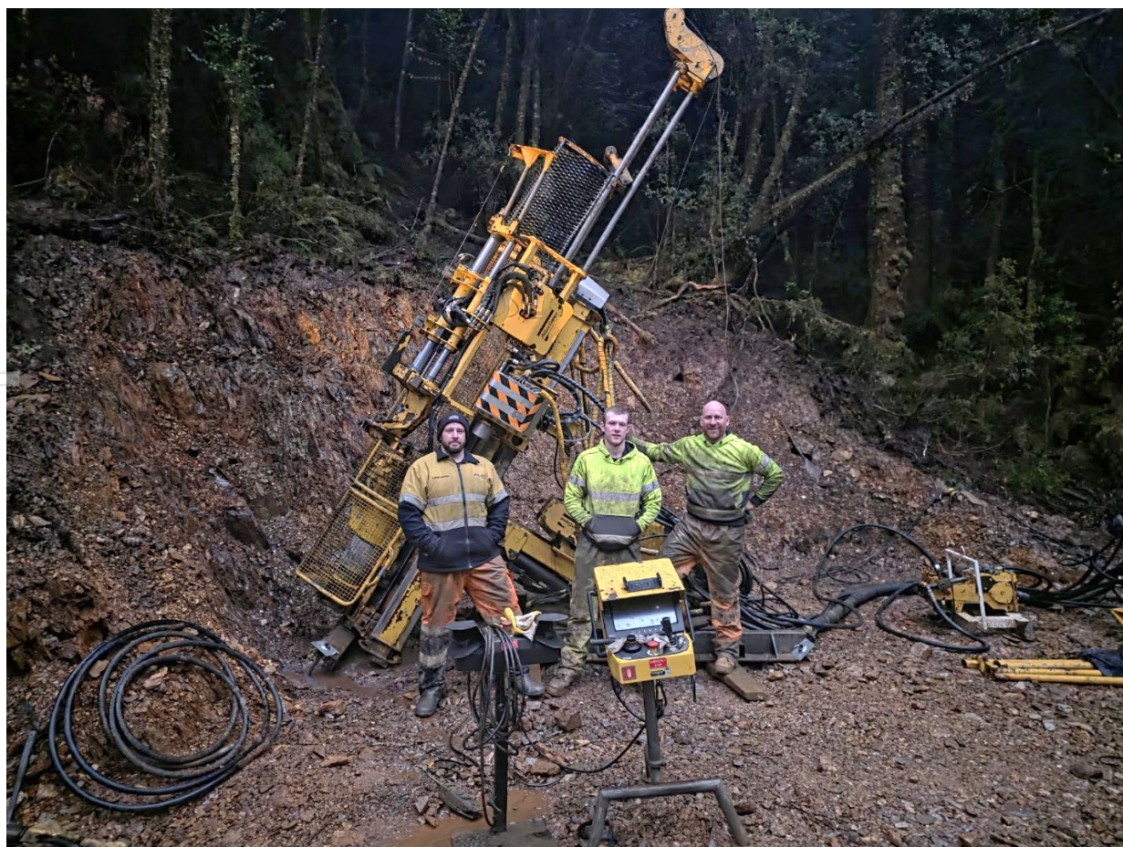
Figure 4 Drilling rig set up on planned hole MZS43 at Montezuma
