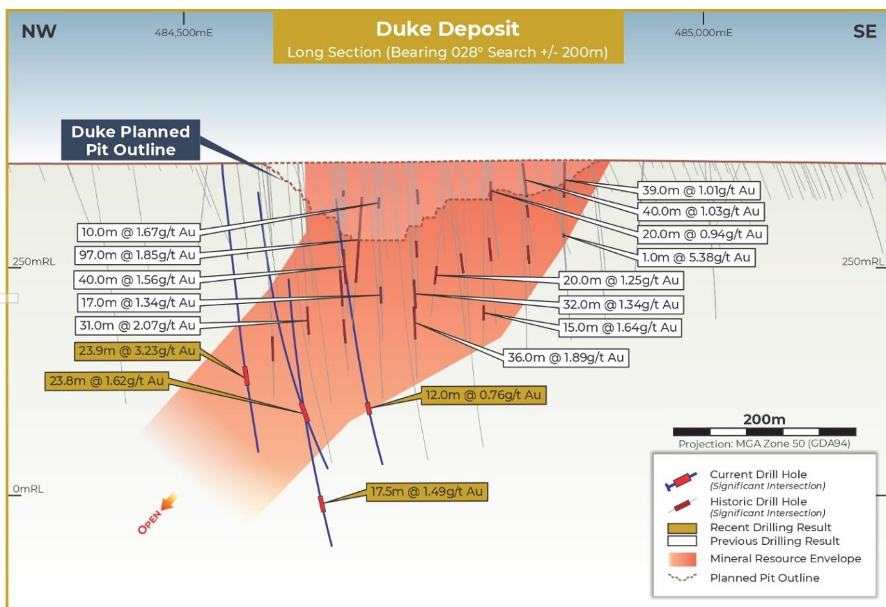
Figure 27: Duke - long section showing recent results
