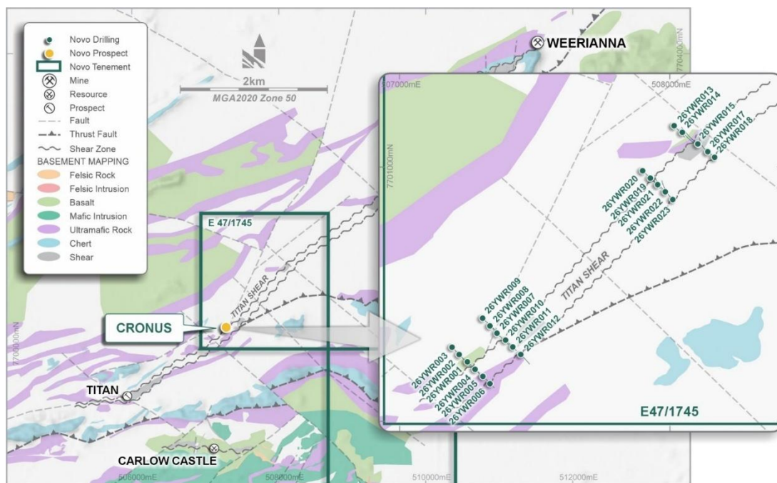
Figure 9. Cronus Gold Prospect tenure showing the regional setting of the Titan shear zone and the Titan prospect and Weerianna deposit. The inset image shows the drill collar locations completed at Cronus.
