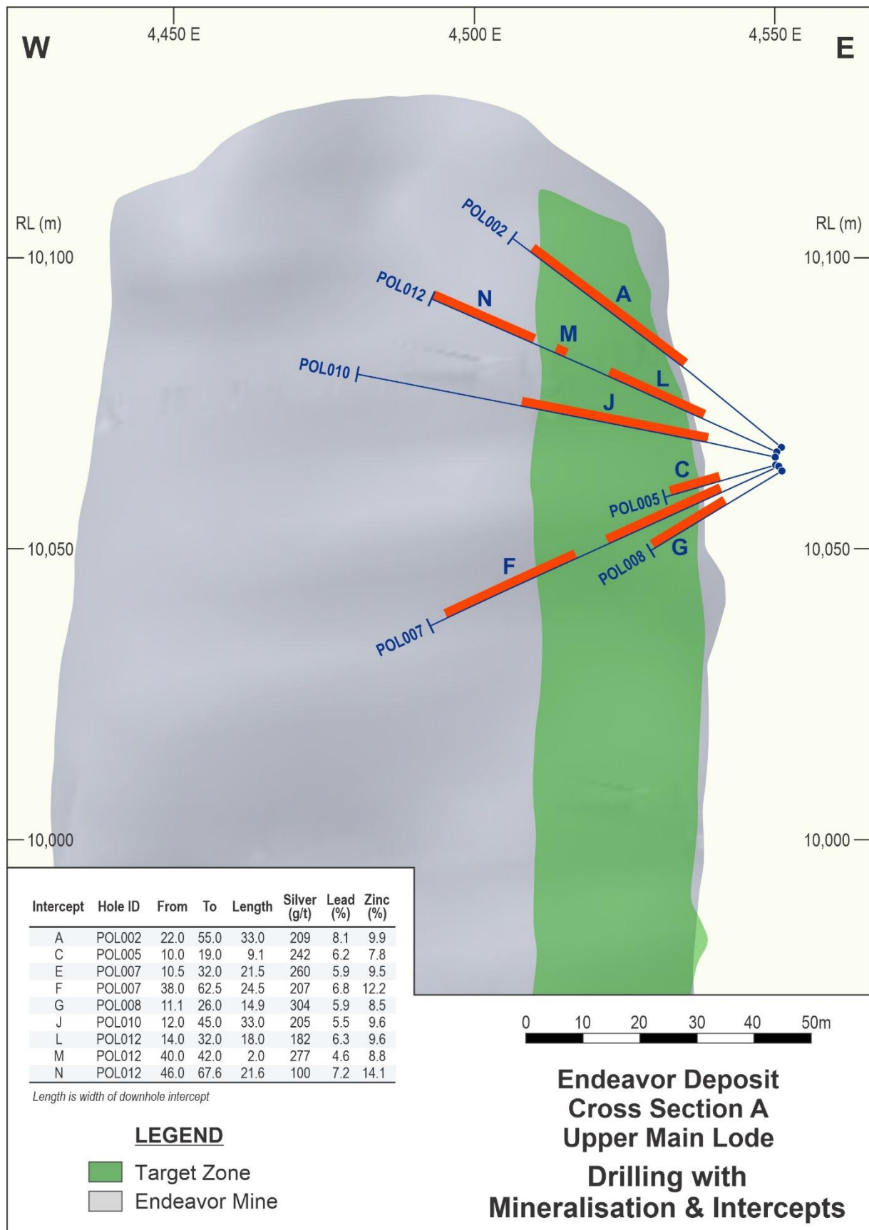
Figure 4. Cross Section A – Upper Main Lode drilling with mineralised intercepts. (previous release)
