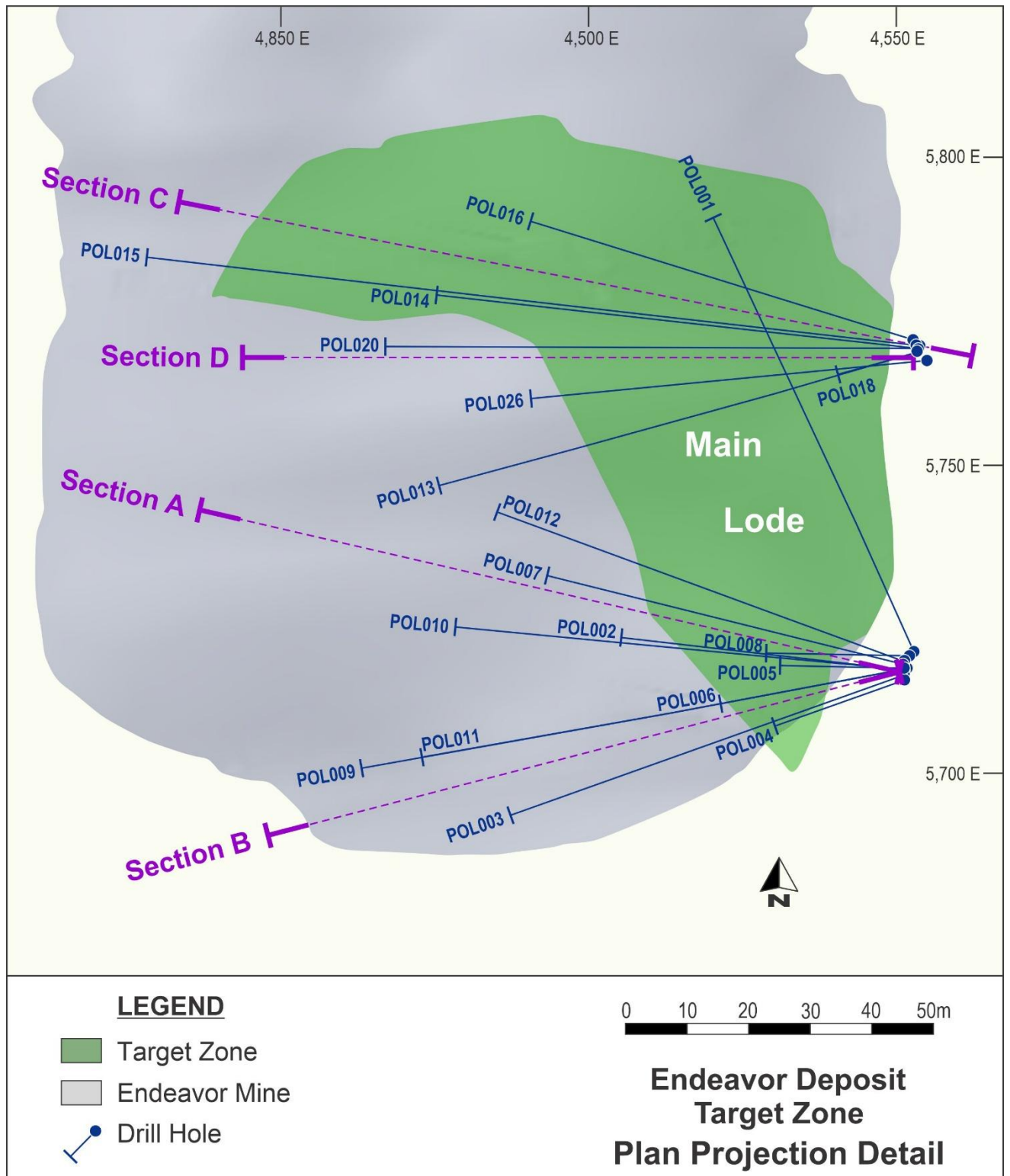
Figure 3. Target Area plan view with surface projection of drilling.
