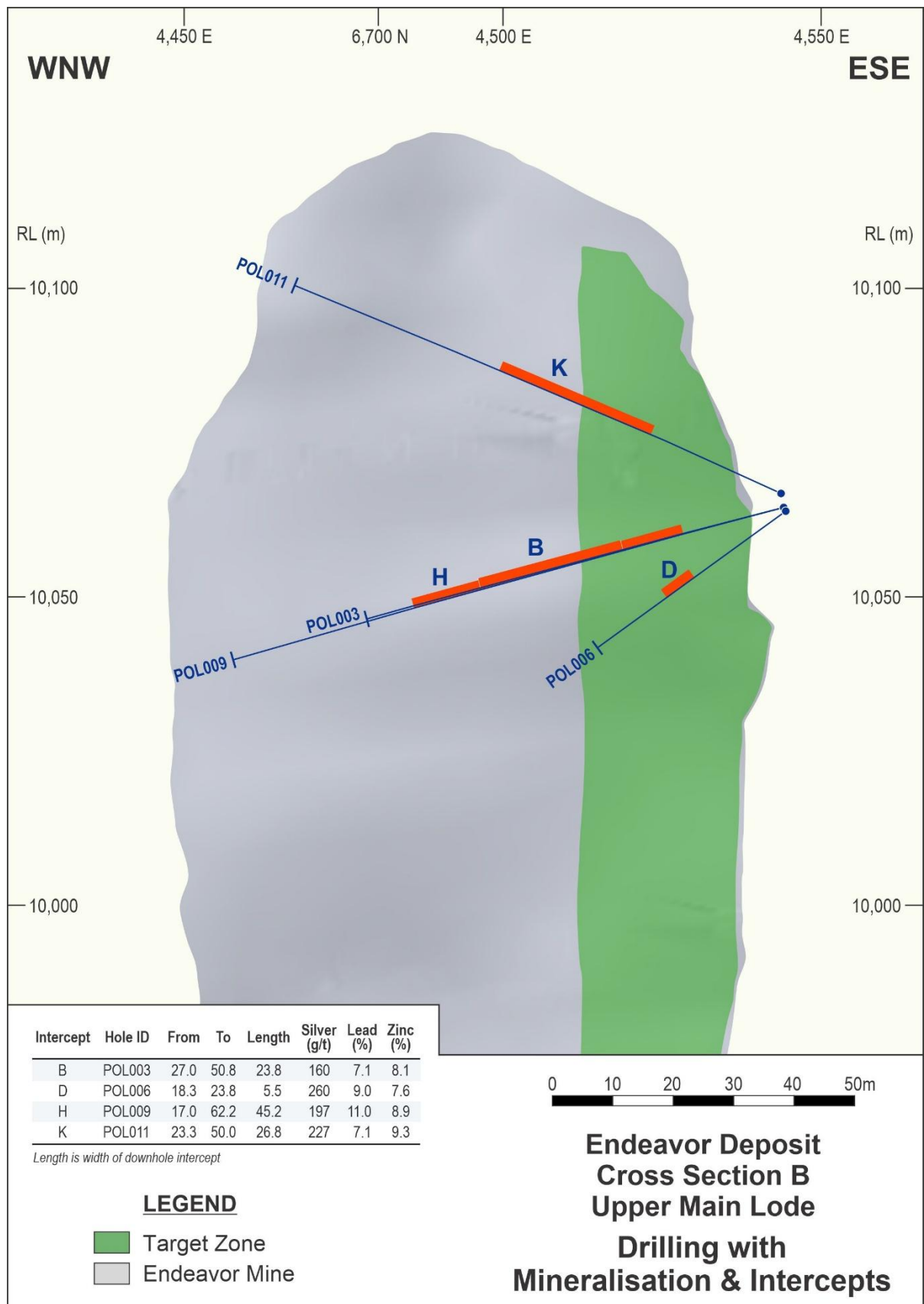
Figure 5. Cross Section B – Upper Main Lode drilling with mineralised intercepts. (previous release)
