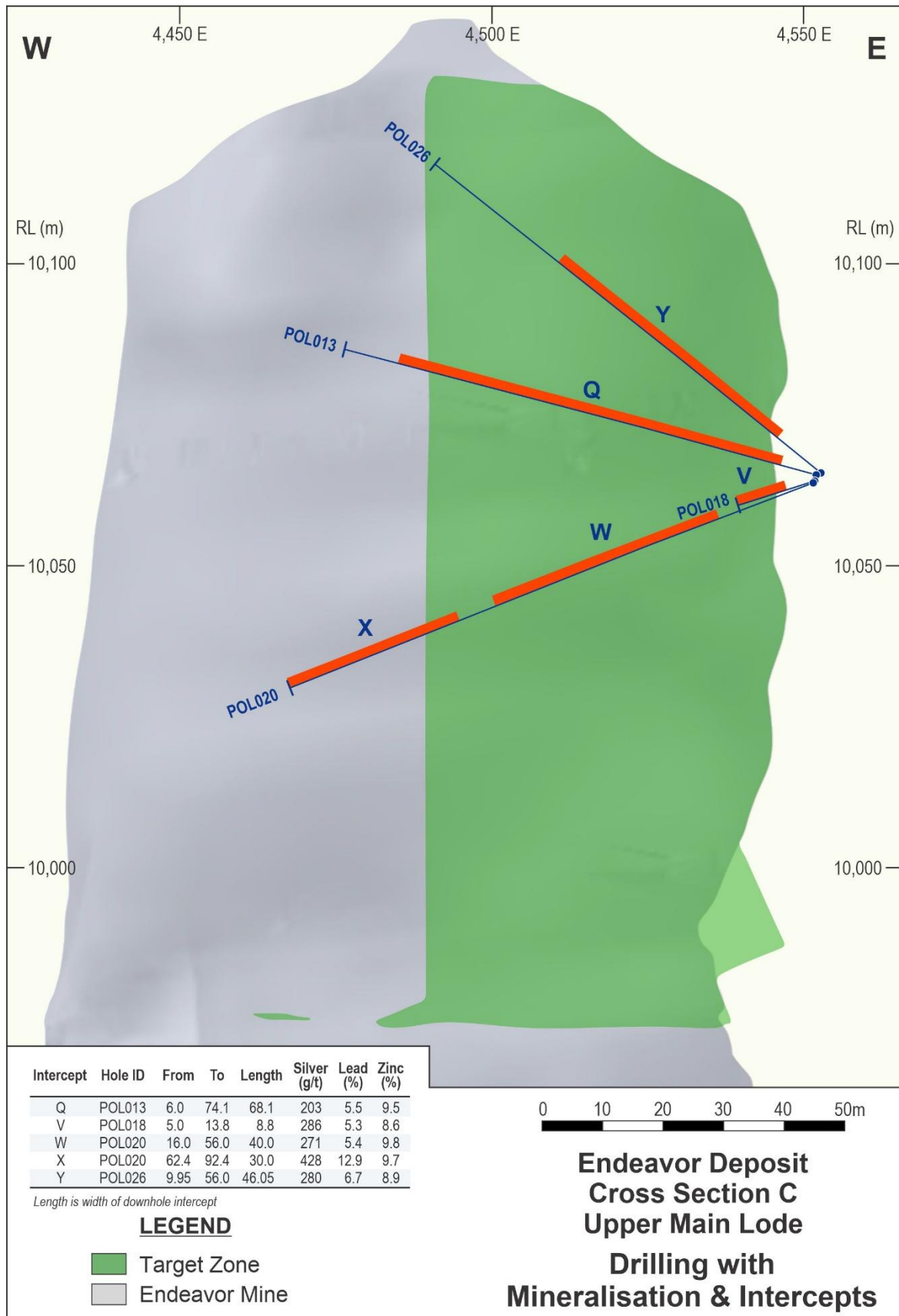
Figure 6. Cross Section C – Upper Main Lode drilling with mineralised intercepts. (this release)
