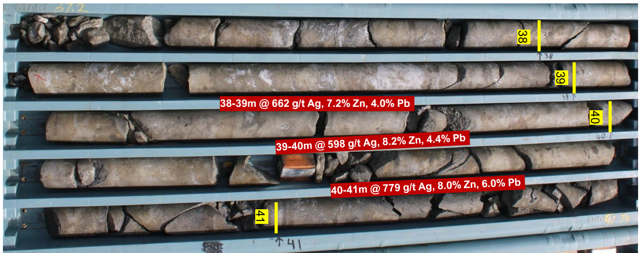
Figure 8: Massive sulphide: POL016 38 – 41 m downhole depth; 3 m @ 680 g/t Ag, 7.8% Zn and 4.8% Pb.
