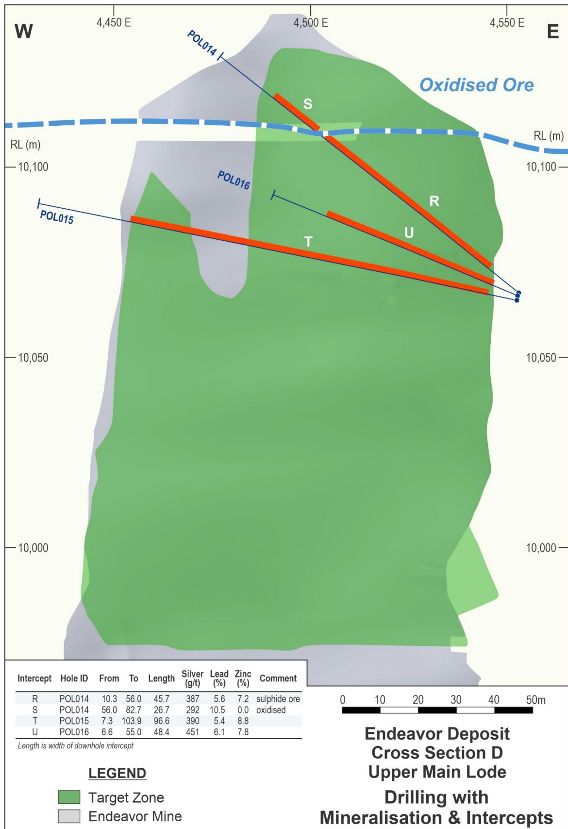
Figure 7. Cross Section D – Upper Main Lode drilling with mineralised intercepts. (this release)
