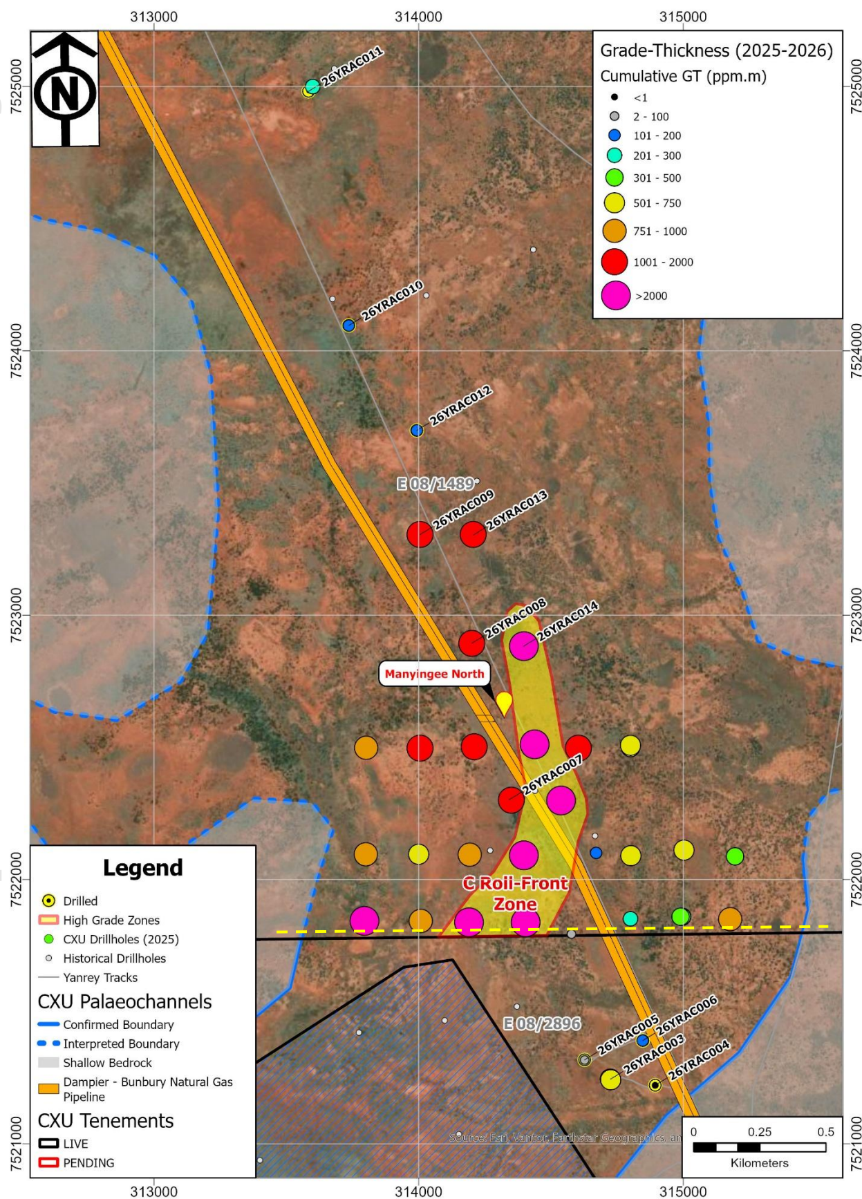
Figure 7. Manyingee North Cumulative GT (ppm*m) map. Dashed line showing location of Cross Section in Figure 6Error! Reference source not found..
