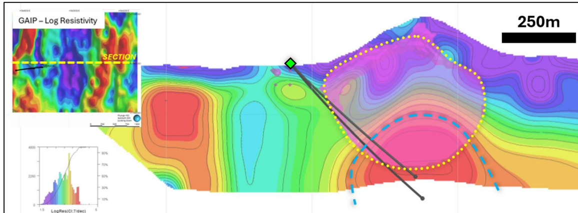
Figure 1. Schematic cross section of the Mt Dillon target showing proposed drill hole traces planned to intercept a >20mV chargeability (yellow dots) and resistivity (blue dash) IP anomaly.
