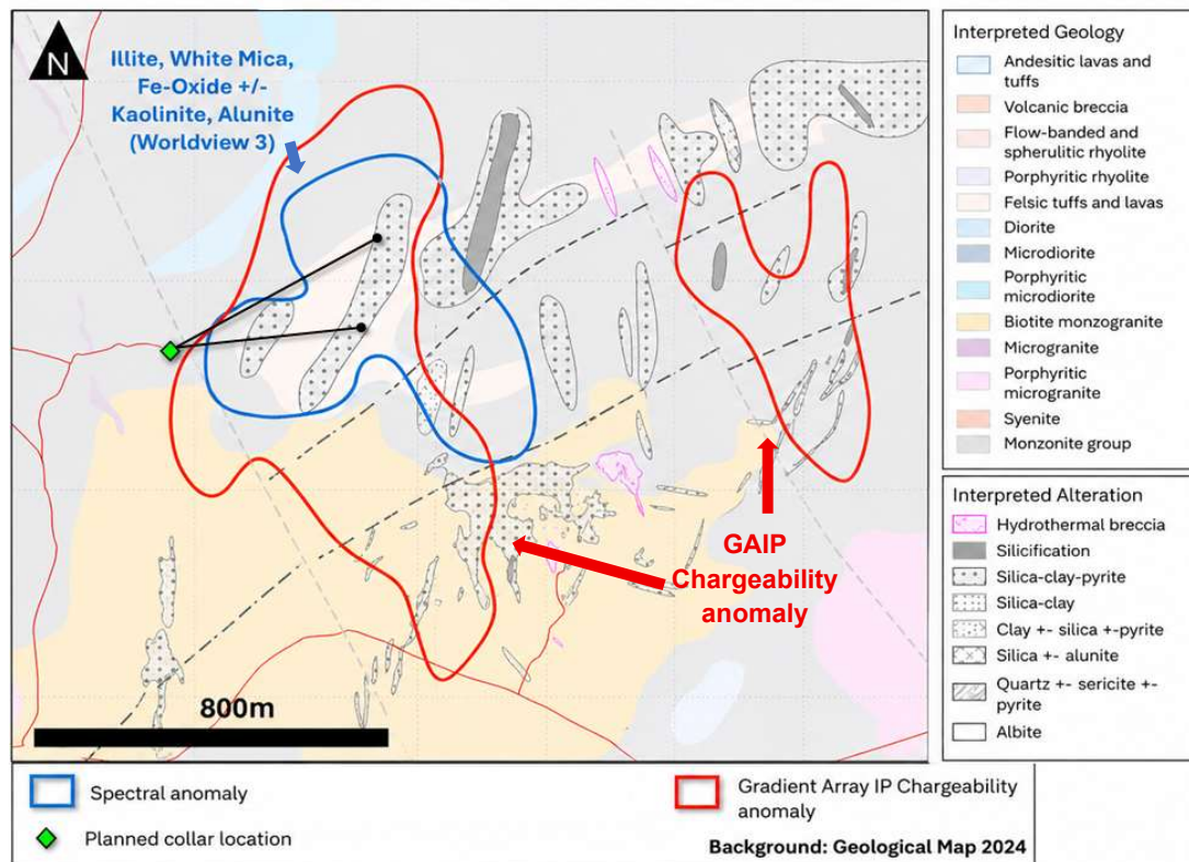
Figure 3. Gradient Array IP anomalies (red) over interpreted geology and alteration at Mt Dillon.
