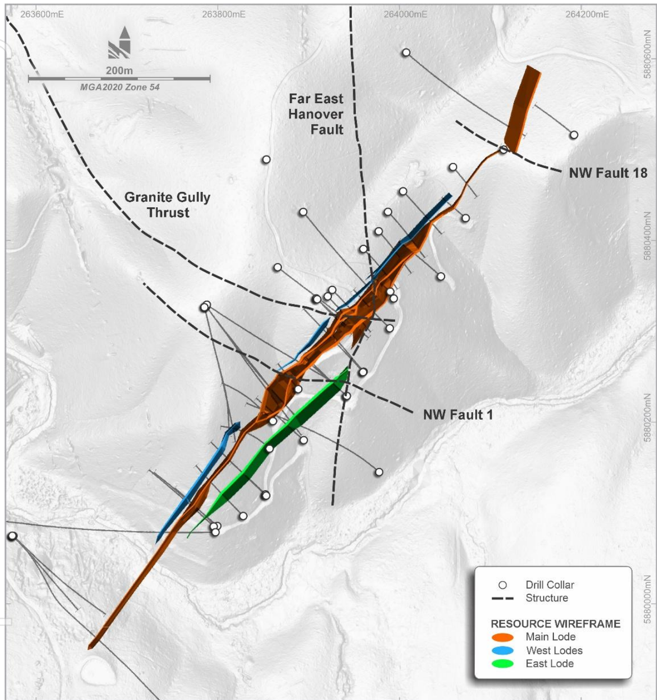
Figure 14.3 Overview of the LSC model
