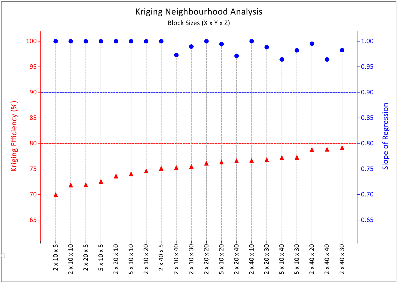
Figure 14.13 KNA plot for block size optimisation
