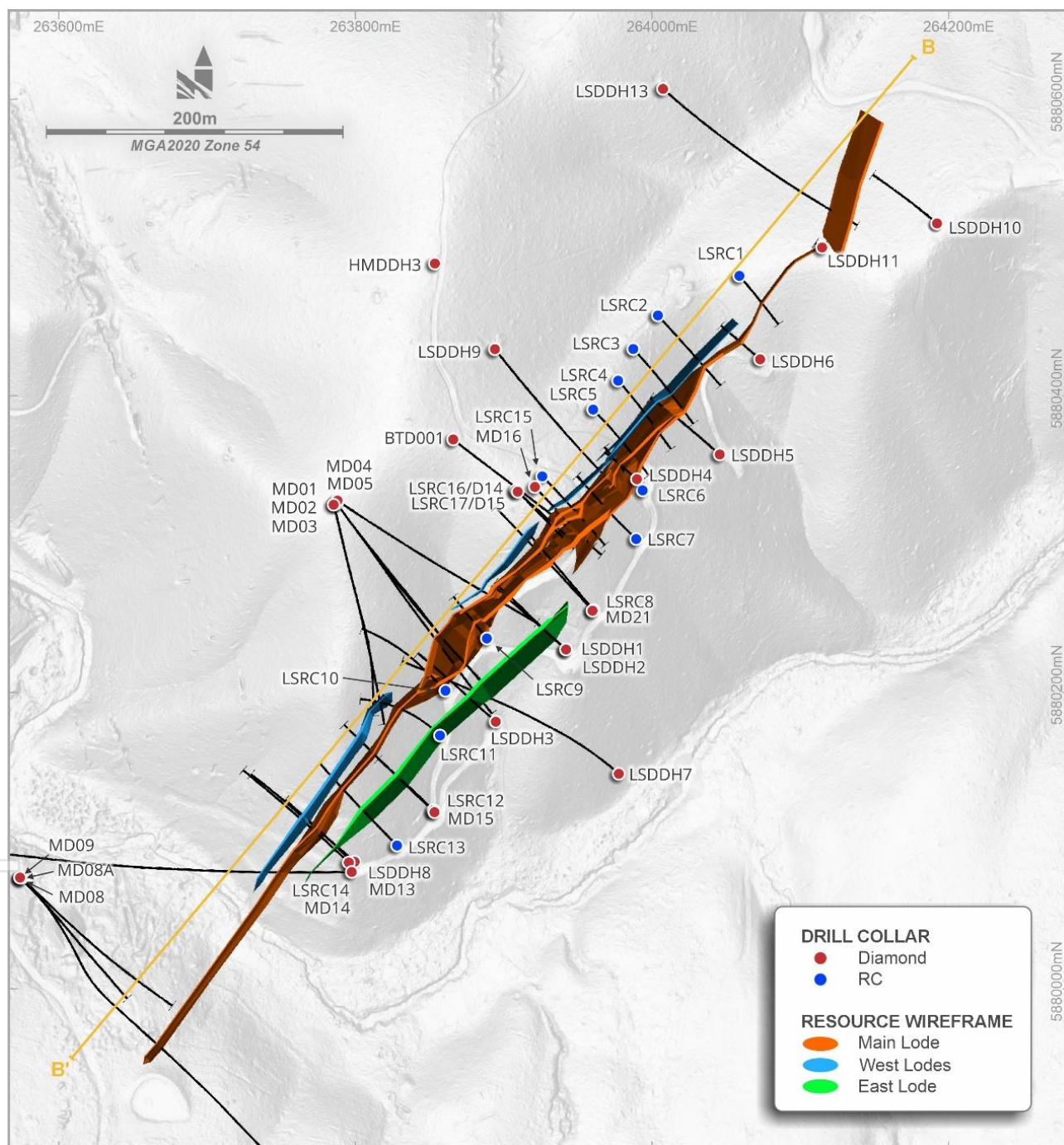
Figure 14.1 LSR collar plan – input drillhole data (model LSC shown)
