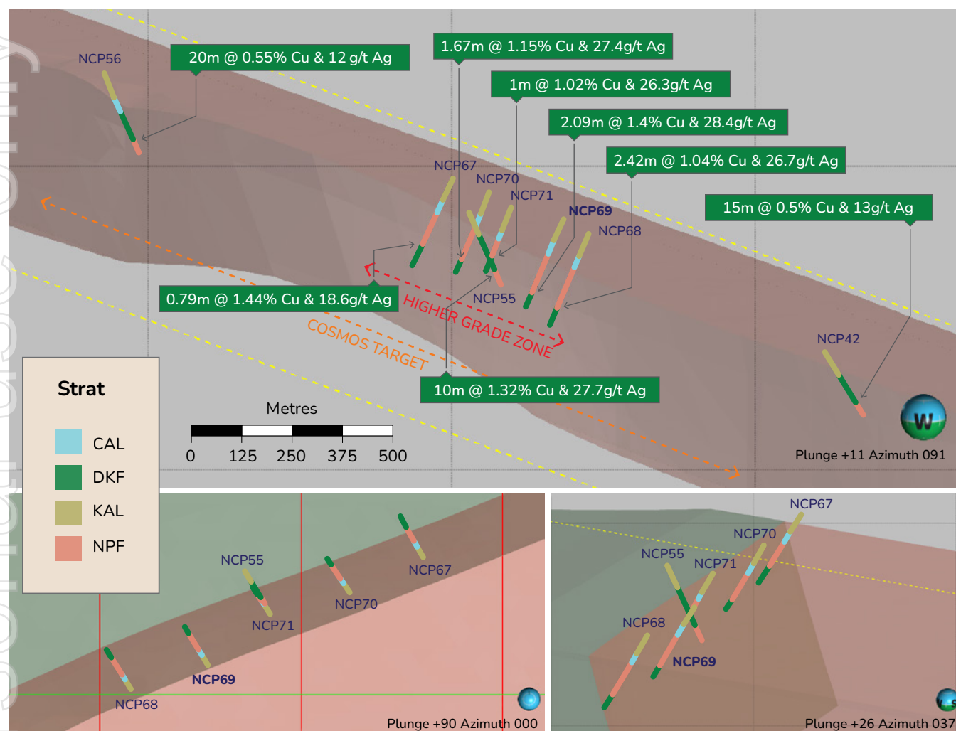
Figure 5 | Oblique 3D section (top and bottom right) and plan (bottom left) illustrating the location of NCP67 to NCP71 in relation to NCP55 and modelled mineralisation. The extent of higher-grade mineralisation intersected in the centre of the Cosmos Target is annotated.
