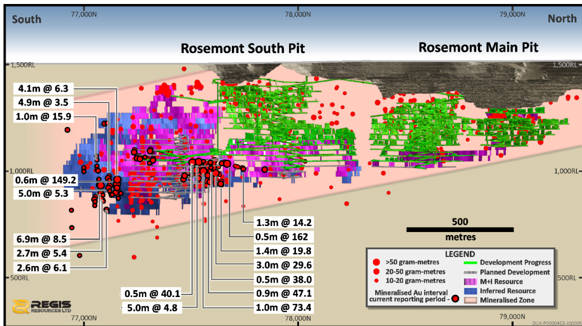
Figure 5: Rosemont long section showing new drill intersections which infill and extend the current resource areas
