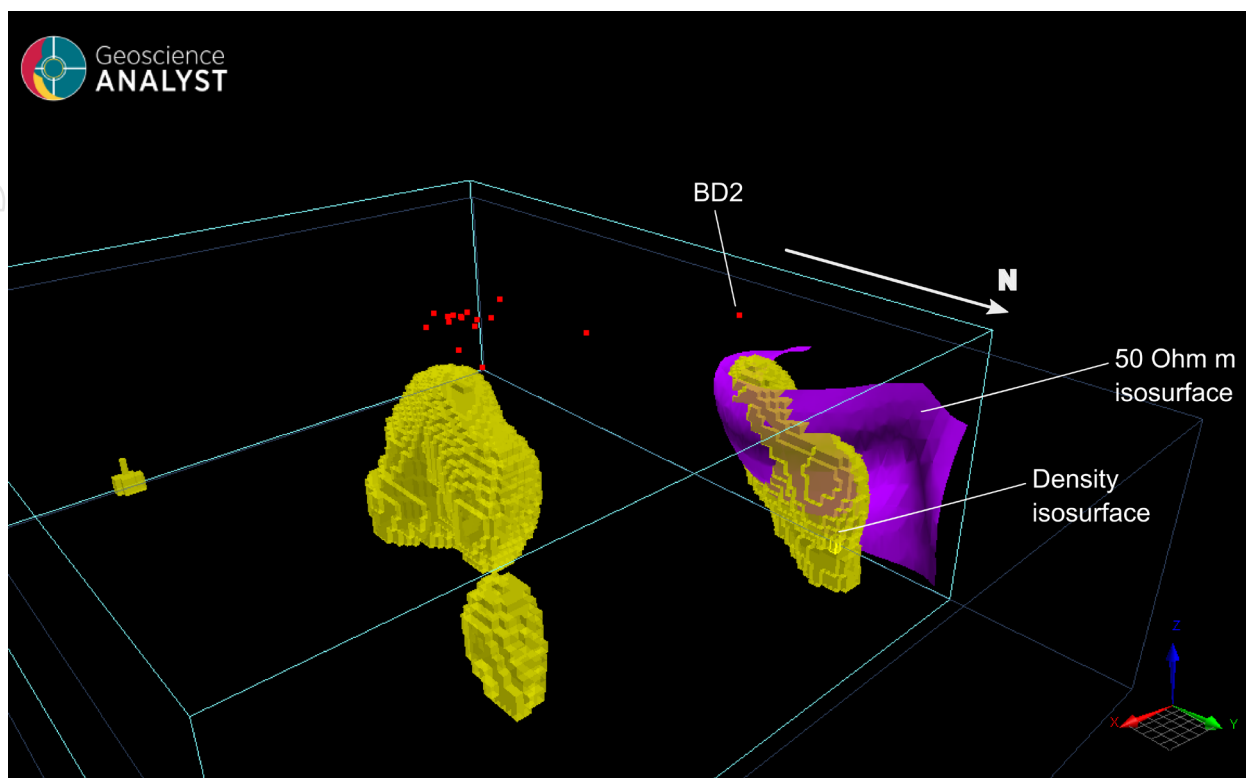
Figure 2. 3D Inversion Model over the Titan Prospect showing iso-surfaces of high-density contrast (yellow bodies), the co-located iso-surface of low resistivity/elevated conductivity (purple body) at Titan West, with location of historic drill holes (red dots). BD2 is the only historic hole at Titan West, drilled by Western Mining Corporation in 1981. (Source: Titan Magnetotellurics, Vox Geophysics, November 2025).
