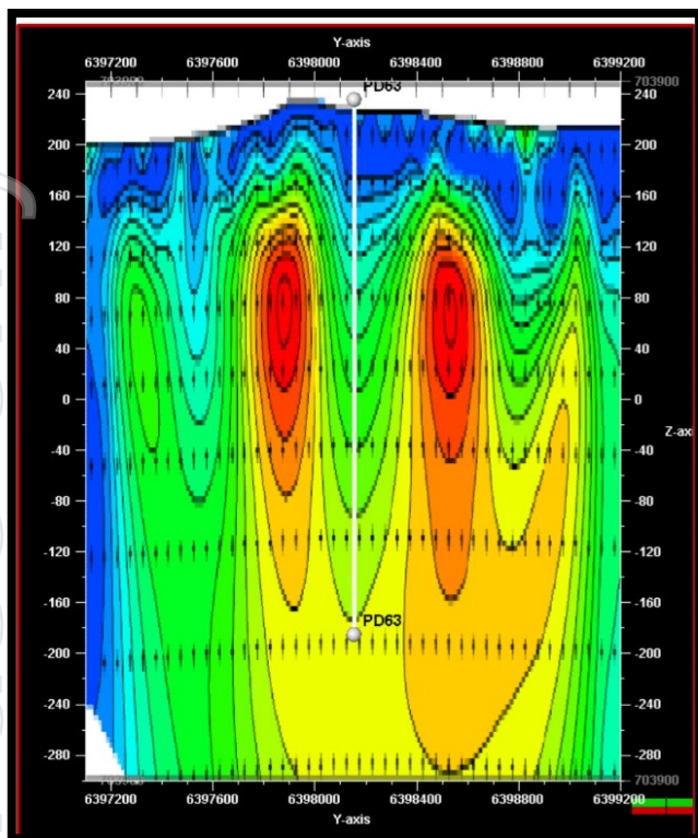
Figure 6c. PD 63 IP Conductivity
