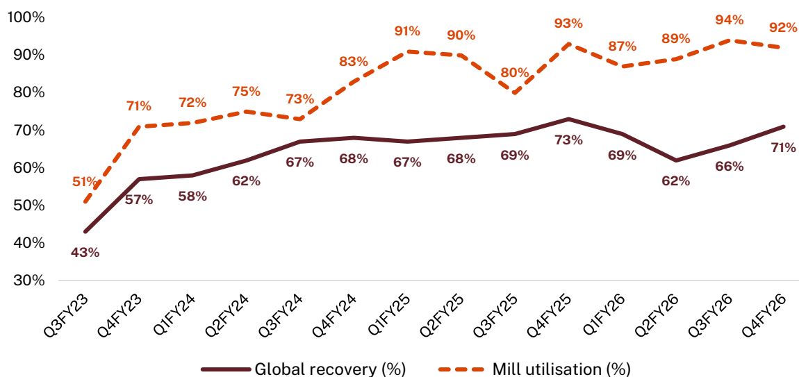
Figure 1: NAL Global Recovery and Mill Utilisation
