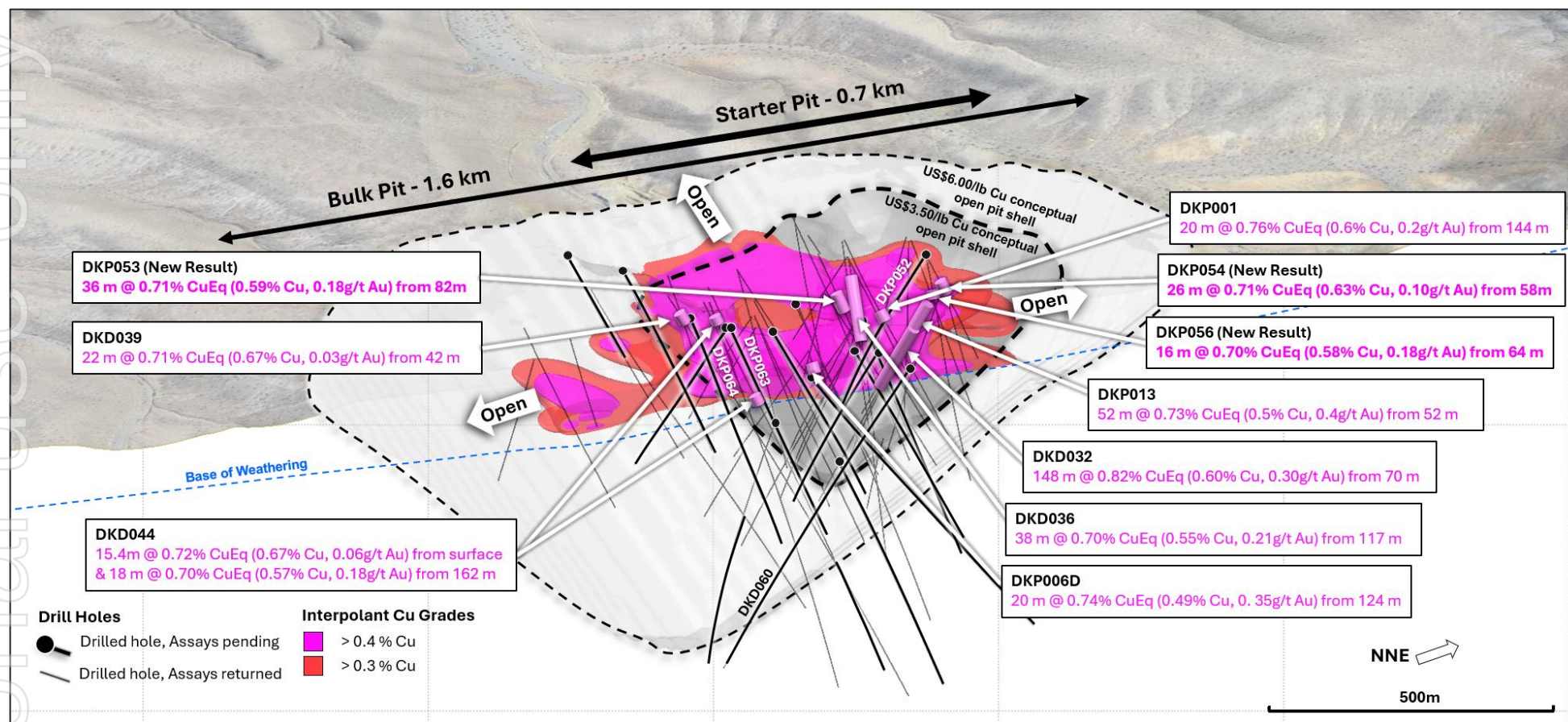
Figure 5. Oblique slice towards NW (Azi 325°, Plunge+26°). 0.3% and 0.4% Cu interpolants displayed for oxide and transitional material, sliced along NNE orientation with the front removed. US$3.50/lb Cu conceptual open pit shell displayed in dark grey; US$6.00/lb Cu conceptual open pit shell displayed in light grey 1 . Base of weathering shown as dashed blue line. Results reported including CuEq 2 .
