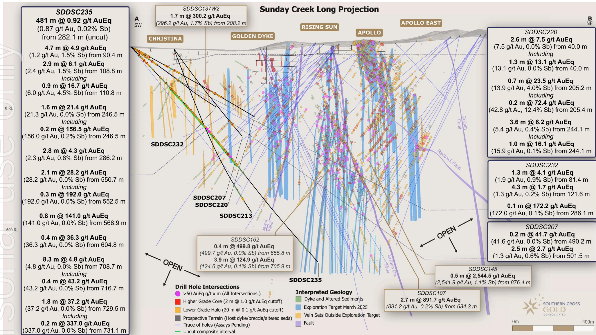
Figure 3: Sunday Creek longitudinal section across A-B in the plane of the dyke breccia/alterd sediment host looking towards the NW (striking 56 degrees) indicating mineralized vein sets. Showing holes SDDSC207, SDDSC213, SDDSC220, SDDSC232 and SDDSC235 reported here (dark blue highlighted box, black trace), with selected intersections and prior reported drill holes. The vertical extents of the vein sets are limited by proximity to drill hole pierce points.
