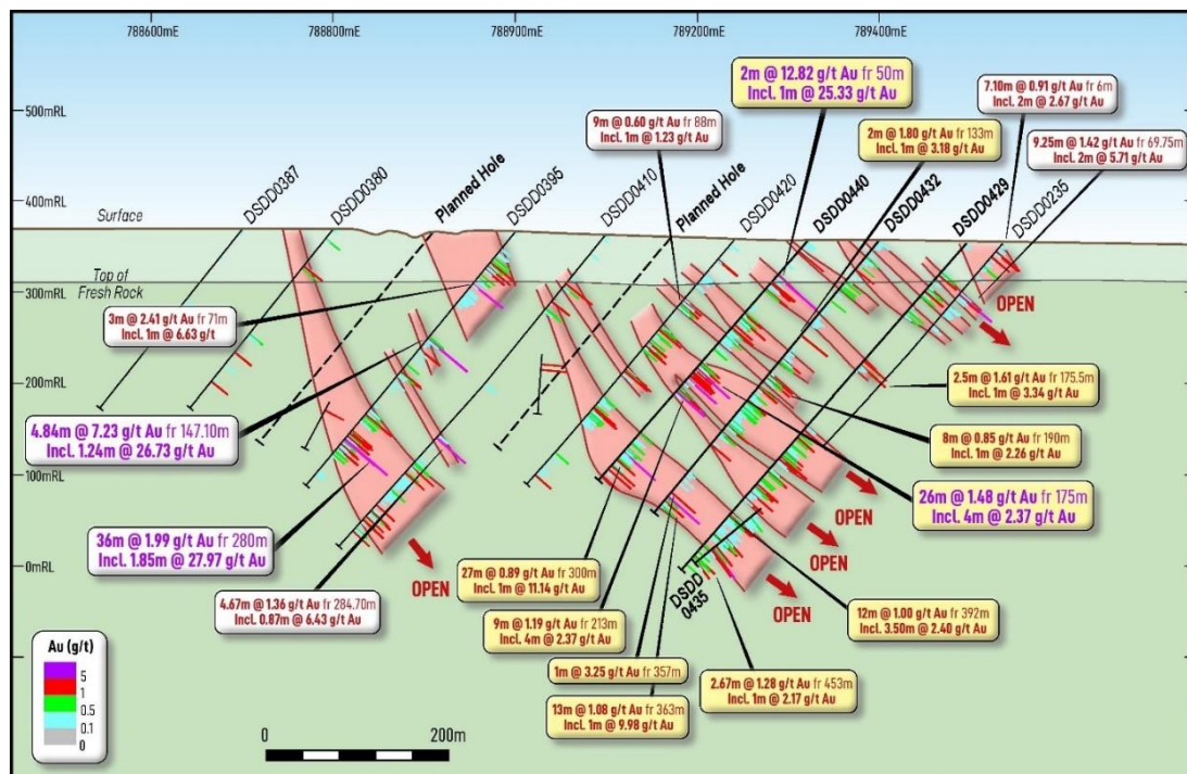
Figure 4: Cross Section looking north (+/-25m) showing new drill results (yellow) for BDT2 4
