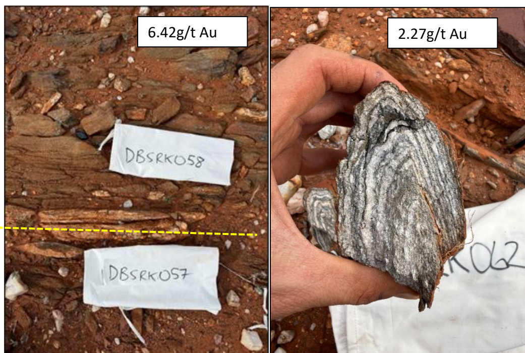
Figure 2 Rock samples confirm bedrock source. DBSRK057 0.34g/t Au, DSRK058 6.42g/t Au and DBSRK062 2.27g/t Au
